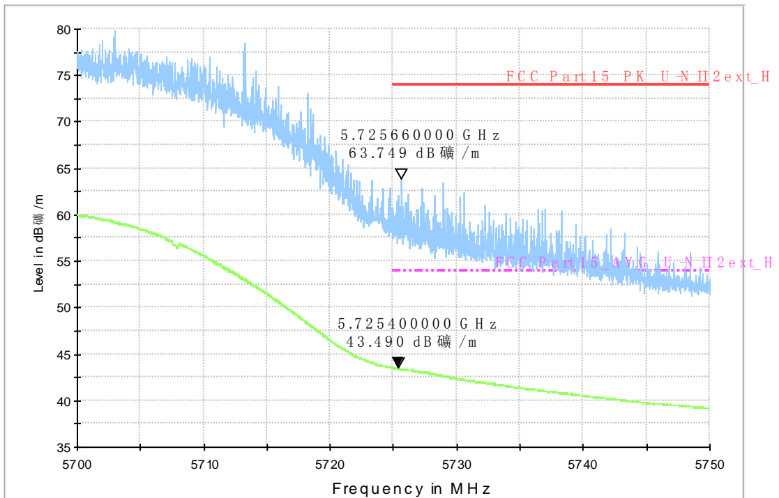
RE - Power-5.70GHz-5.75GHz
