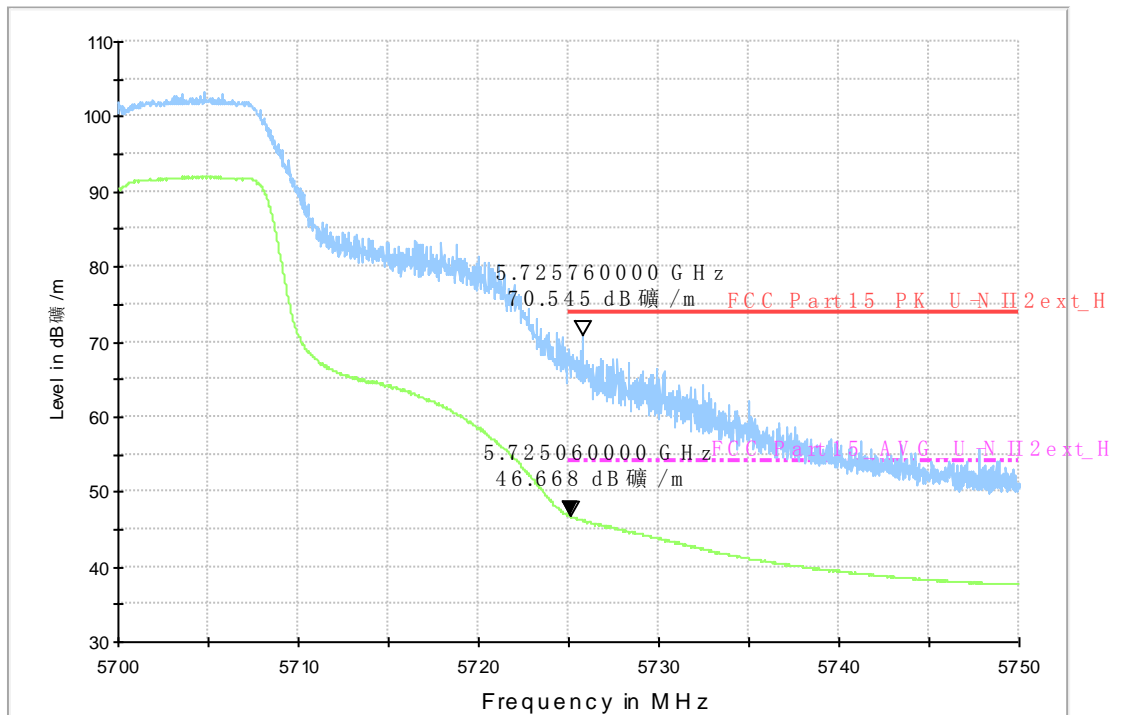
RE - Power-5.70GHz-5.75GHz
