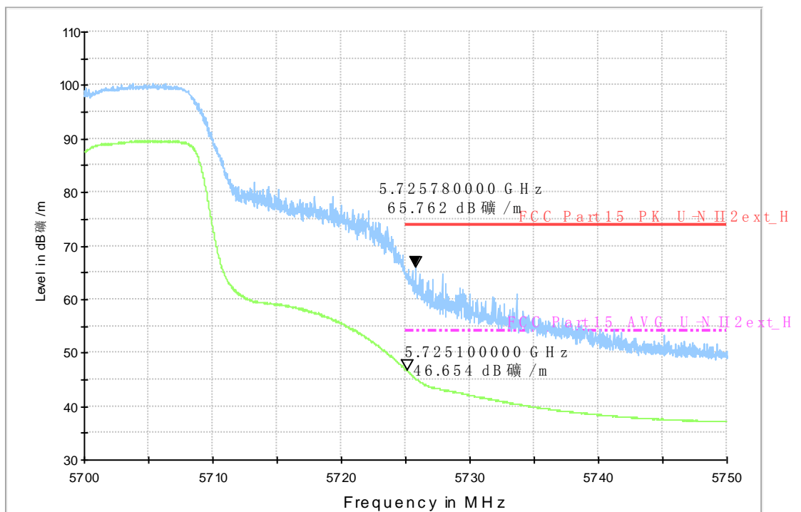
RE - Power-5.70GHz-5.75GHz
