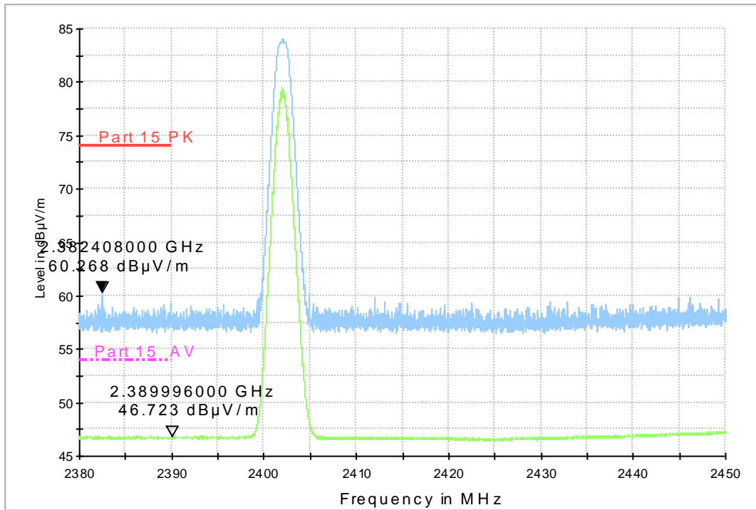
Fig.1. Transmitter Spurious Emission - Radiated (Power): GFSK low channel
