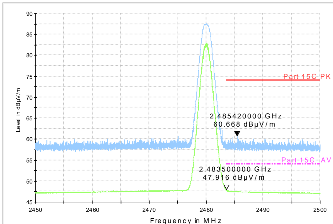
Fig.2. Transmitter Spurious Emission - Radiated (Power): GFSK high channel
