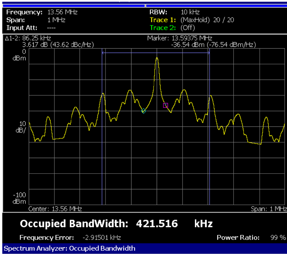
Figure A-10: Test result of EUT1 at test set. NFC02
