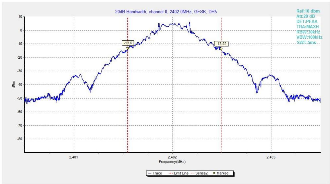
Fig.107. 20dB Bandwidth: GFSK, Channel 0
