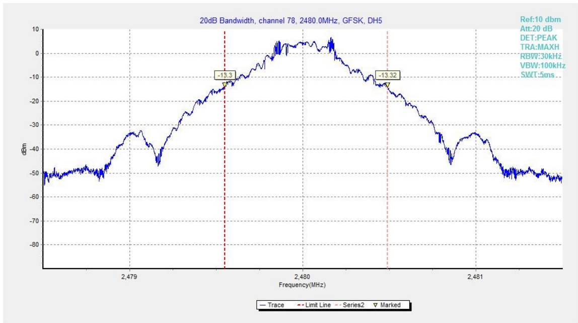
Fig.109. 20dB Bandwidth: GFSK, Channel 78
