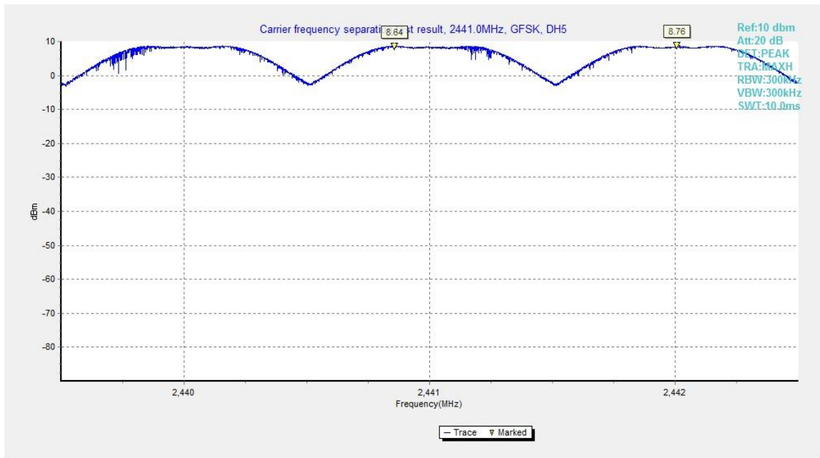
Fig.116. Carrier frequency separation measurement: GFSK, Channel 39
