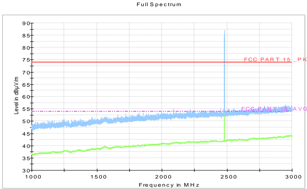
Fig.24. Transmitter Spurious Emission - Radiated: GFSK, 2480MHz, 1 GHz - 3 GHz
