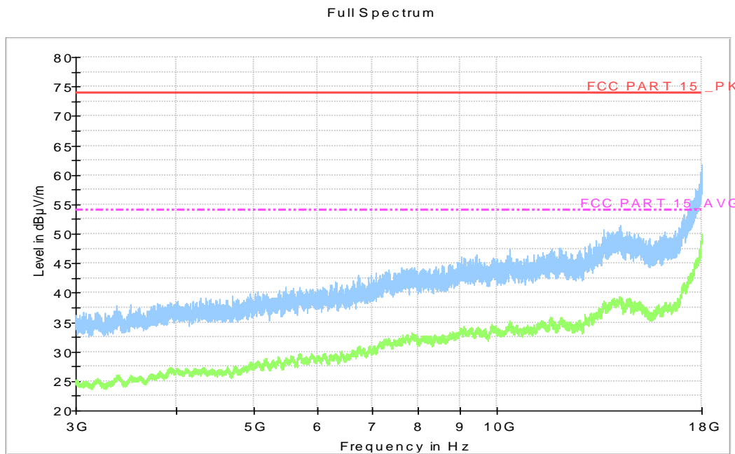
Fig.25. Transmitter Spurious Emission - Radiated: GFSK, 2480MHz, 3 GHz - 18 GHz
