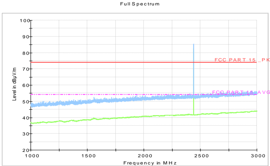
Fig.22. Transmitter Spurious Emission - Radiated: GFSK, 2440MHz, 1 GHz - 3 GHz
