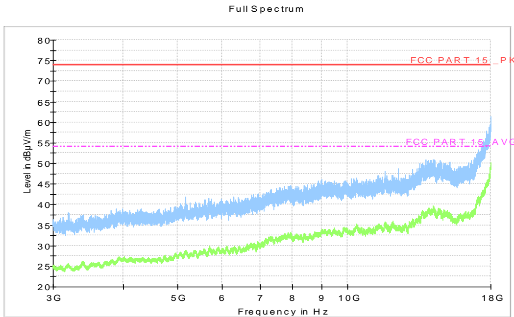
Fig.23. Transmitter Spurious Emission - Radiated: GFSK, 2440MHz, 3 GHz - 18 GHz
