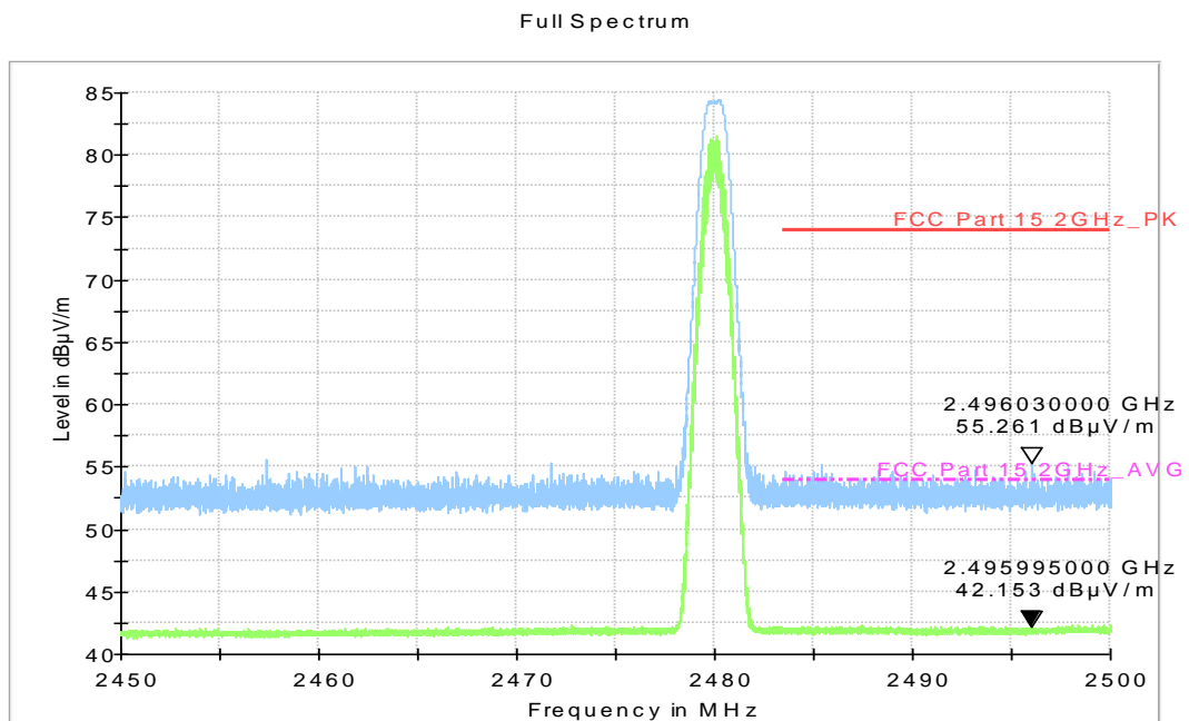
Fig.27. Transmitter Spurious Emission - Radiated (Power): GFSK high channel
