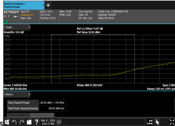
N77(100M)_DFT-s-OFDM_QPSK_Edge_1RB_Left_Low_CH_CHP_PA
