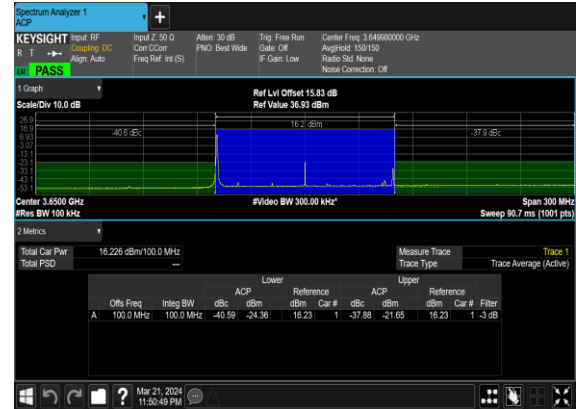
N77(100M)_DFT-s-OFDM_PI_2-BPSK_Edge_1RB_Left_High_CH
