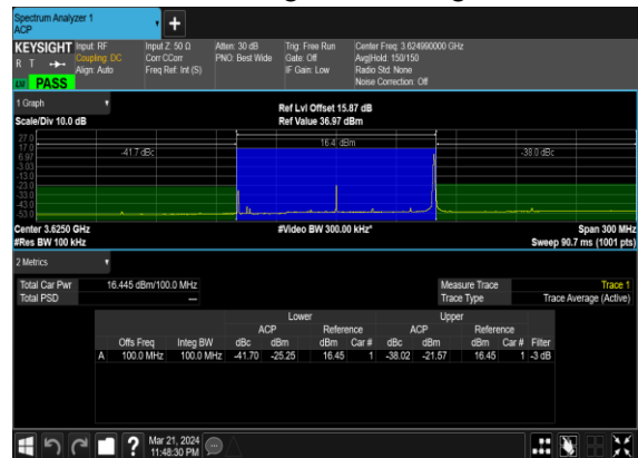
N77(100M)_DFT-s-OFDM_QPSK_Edge_1RB_Right_Mid_CH
