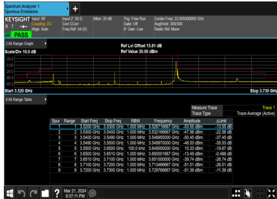
N77(100M)_DFT-s-OFDM_QPSK_Edge_1RB_Right_Low_CH
