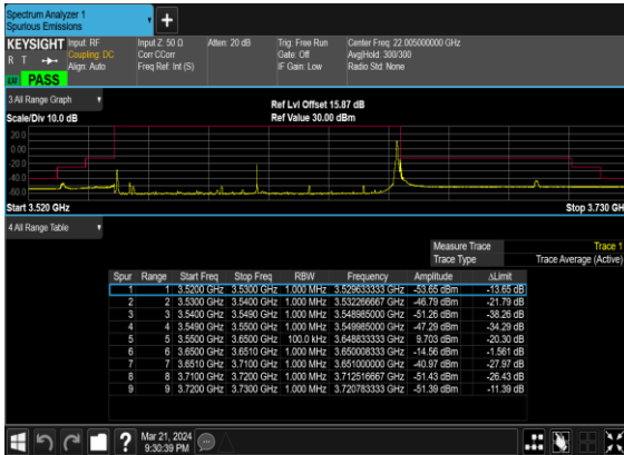
N77(100M)_DFT-s-OFDM_BPSK_Edge_1RB_Right_Low_CH
