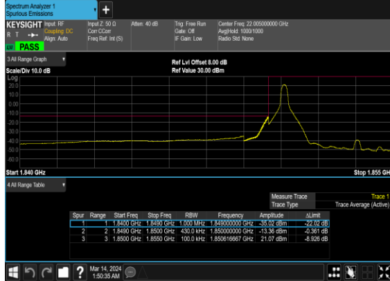
N2(40M)_DFT-s- OFDM_QPSK_Edge_1RB_Left_Low_CH
