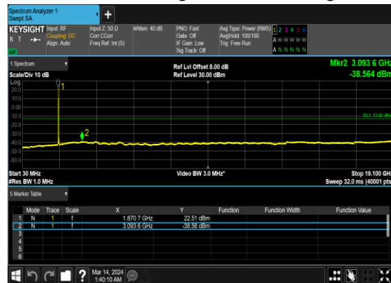
N2(40M)_DFT-s- OFDM_QPSK_Edge_1RB_Left_High_CH
