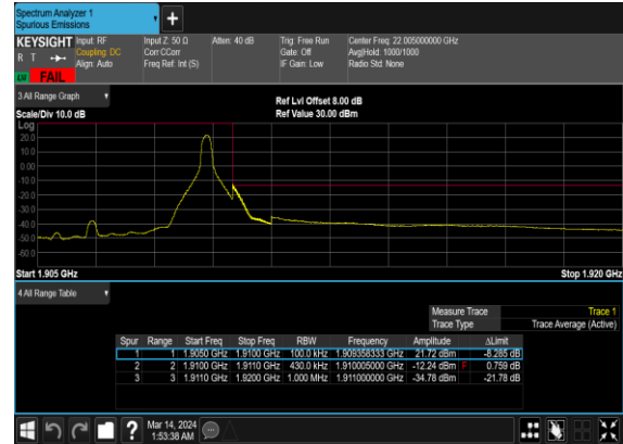
N2(40M)_DFT-s- OFDM_BPSK_Edge_1RB_Right_High_CH
