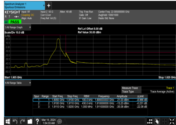
N2(40M)_DFT-s- OFDM_QPSK_Edge_1RB_Right_High_CH
