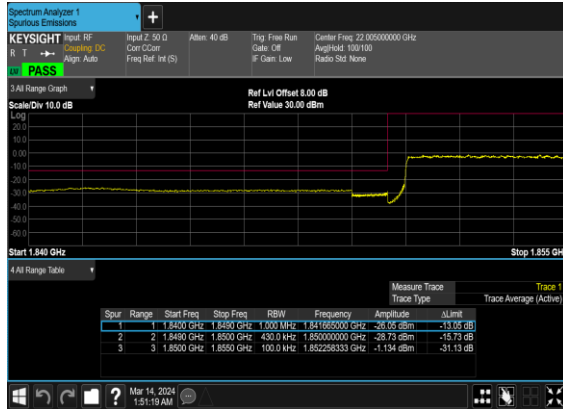
N2(40M)_DFT-s- OFDM_QPSK_Outer_Full_Low_CH
