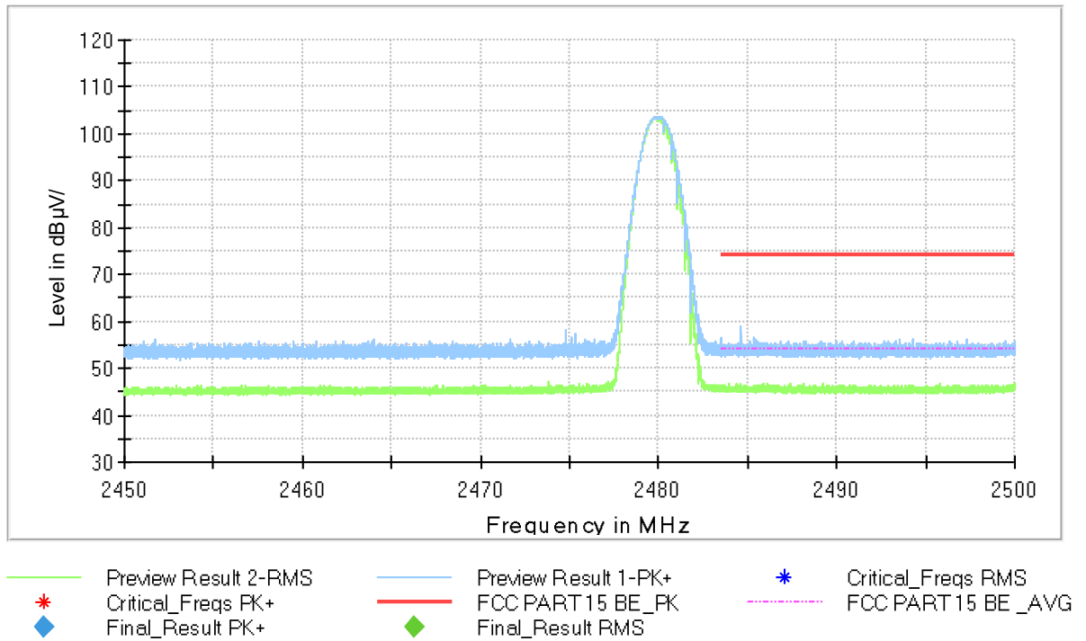
Fig.59. Frequency Band Edges: GFSK, Channel 78, Hopping Off, ch11, 2.45 GHz - 2.50GHz
