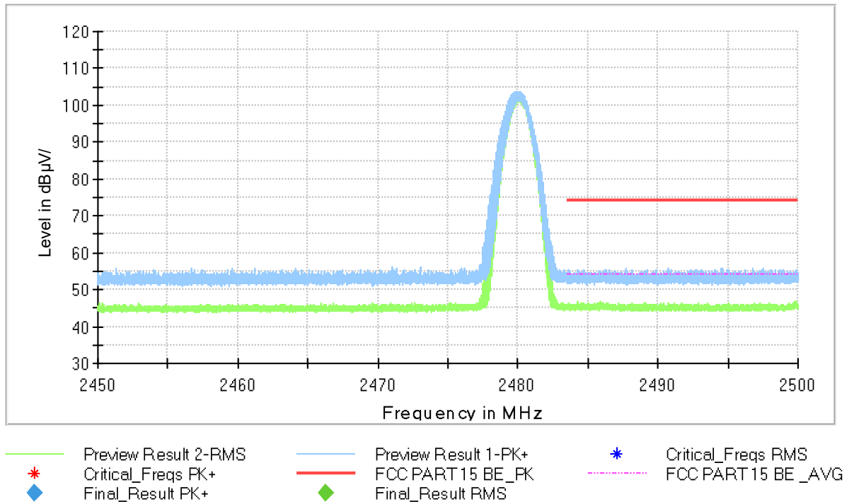
Fig.61. Frequency Band Edges: \pi/4 DQPSK, Channel 78, Hopping Off, 2.45 GHz - 2.50GHz
