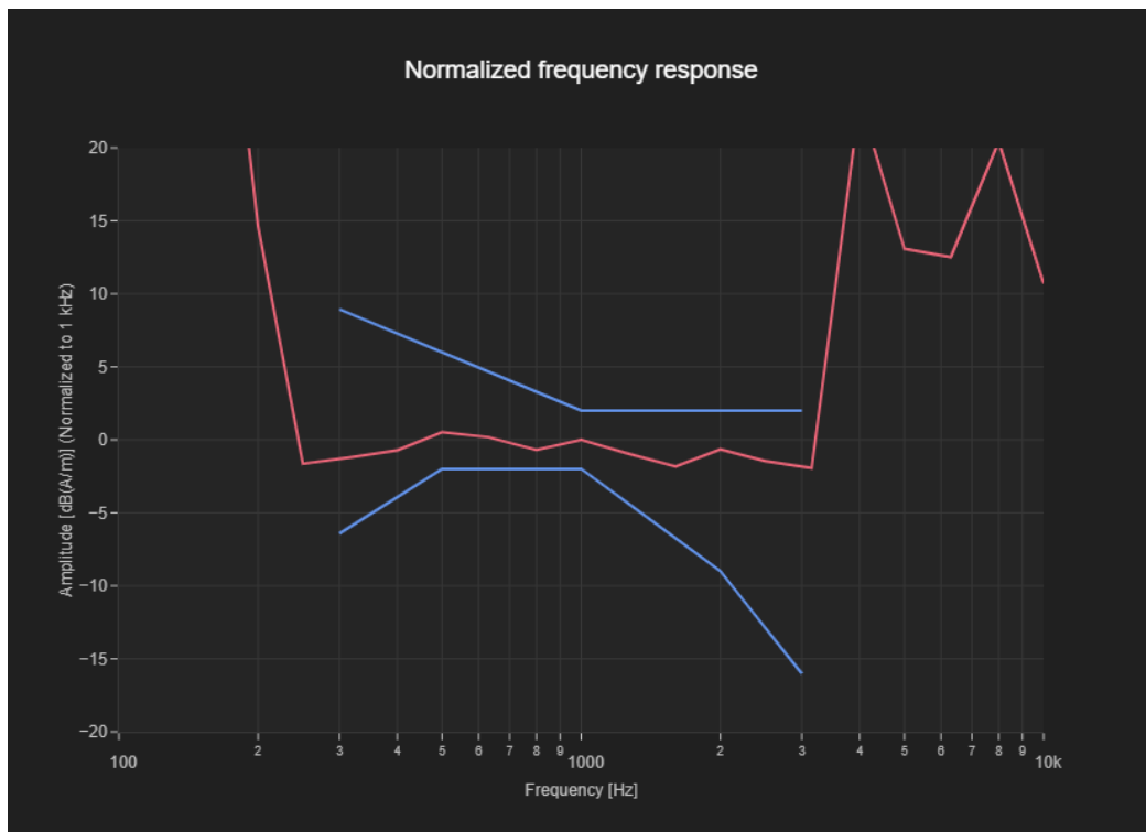
Figure.4 Frequency Response of N25-OTT
