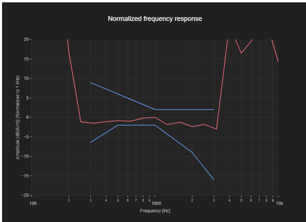
Figure C.4 Frequency Response of N25-OTT
