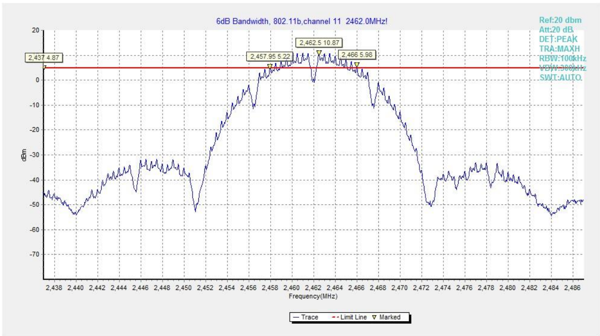
Fig.A.4.3 DTS Bandwidth (802.11b, Ch 11)
