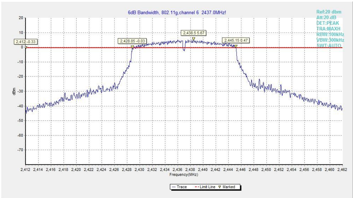
Fig.A.4.5 DTS Bandwidth (802.11g, Ch 6)
