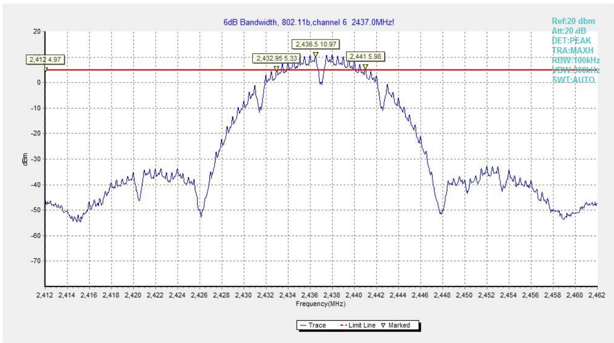
Fig.A.4.2 DTS Bandwidth (802.11b, Ch 6)
