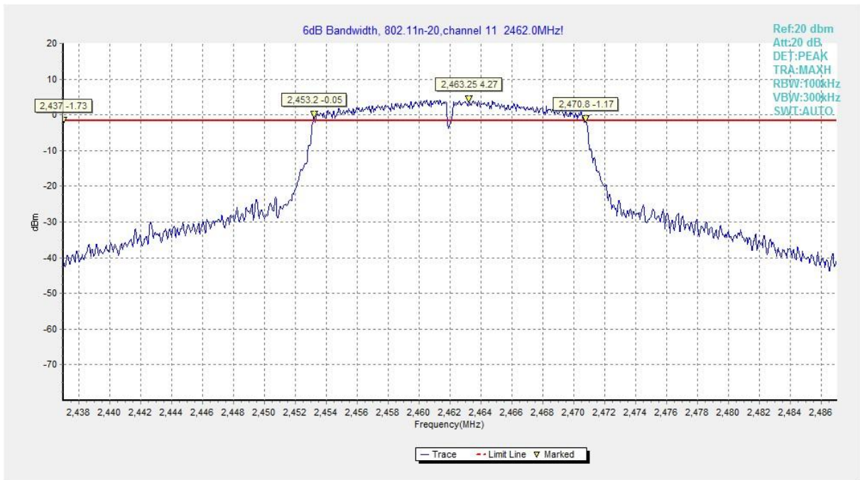
Fig.A.4.9 DTS Bandwidth (802.11n-HT20, Ch 11)
