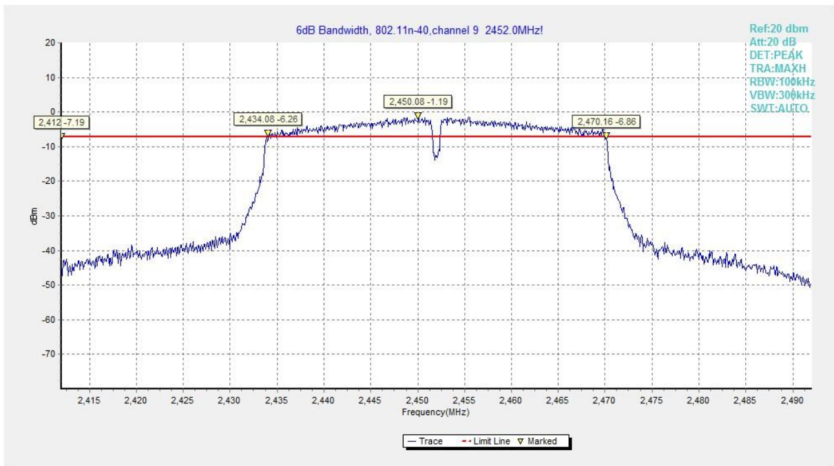
Fig.A.4.12 DTS Bandwidth (802.11n-HT40, Ch 9)
