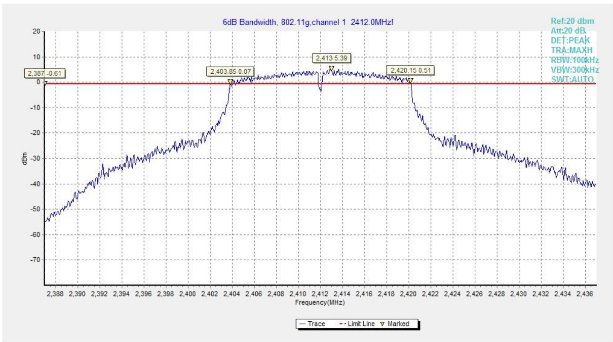
Fig.A.4.4 DTS Bandwidth (802.11g, Ch 1)
