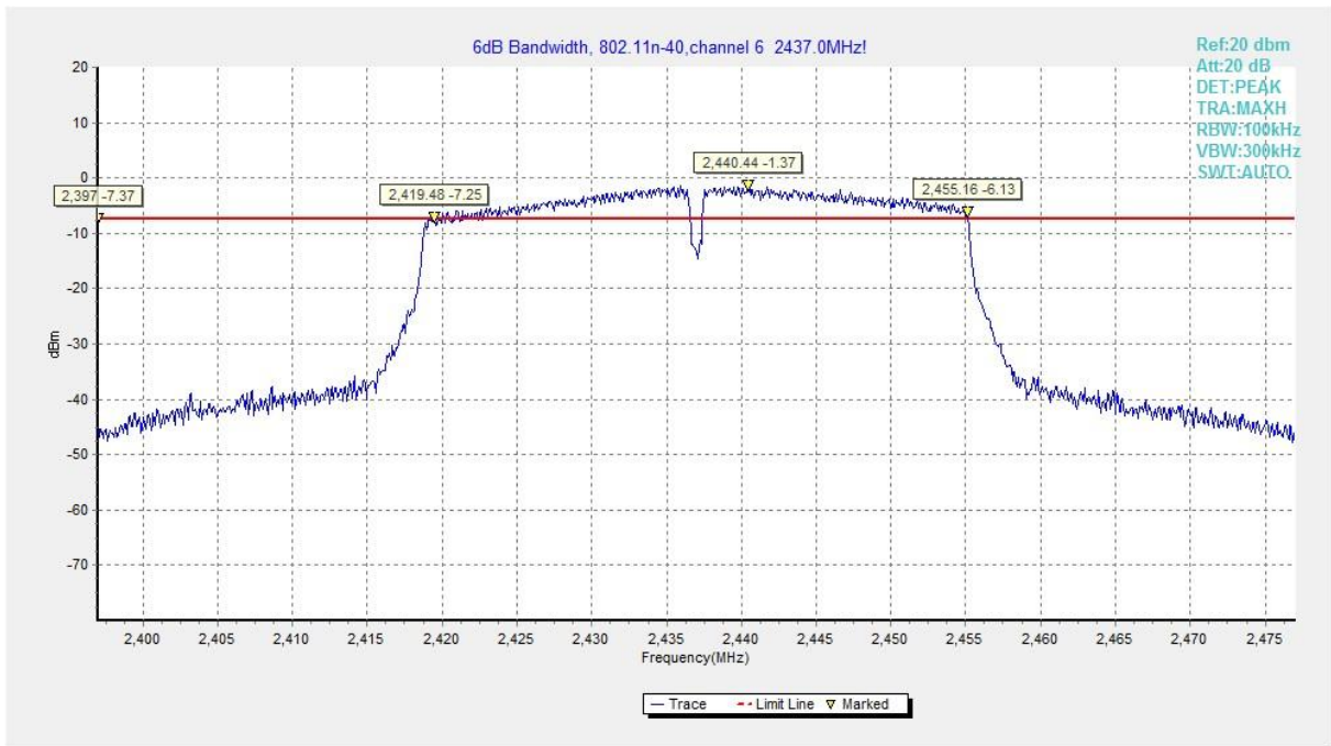
Fig.A.4.11 DTS Bandwidth (802.11n-HT40, Ch 6)
