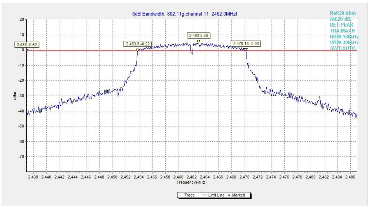
Fig.A.4.6 DTS Bandwidth (802.11g, Ch 11)
