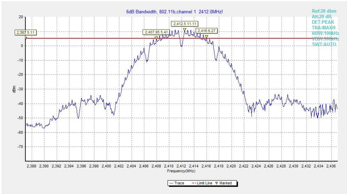
Fig.A.4.1 DTS Bandwidth(802.11b,Ch 1)
