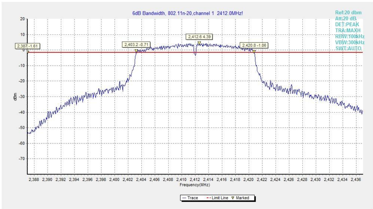
Fig.A.4.7 DTS Bandwidth (802.11n-20MHz, Ch 1)
