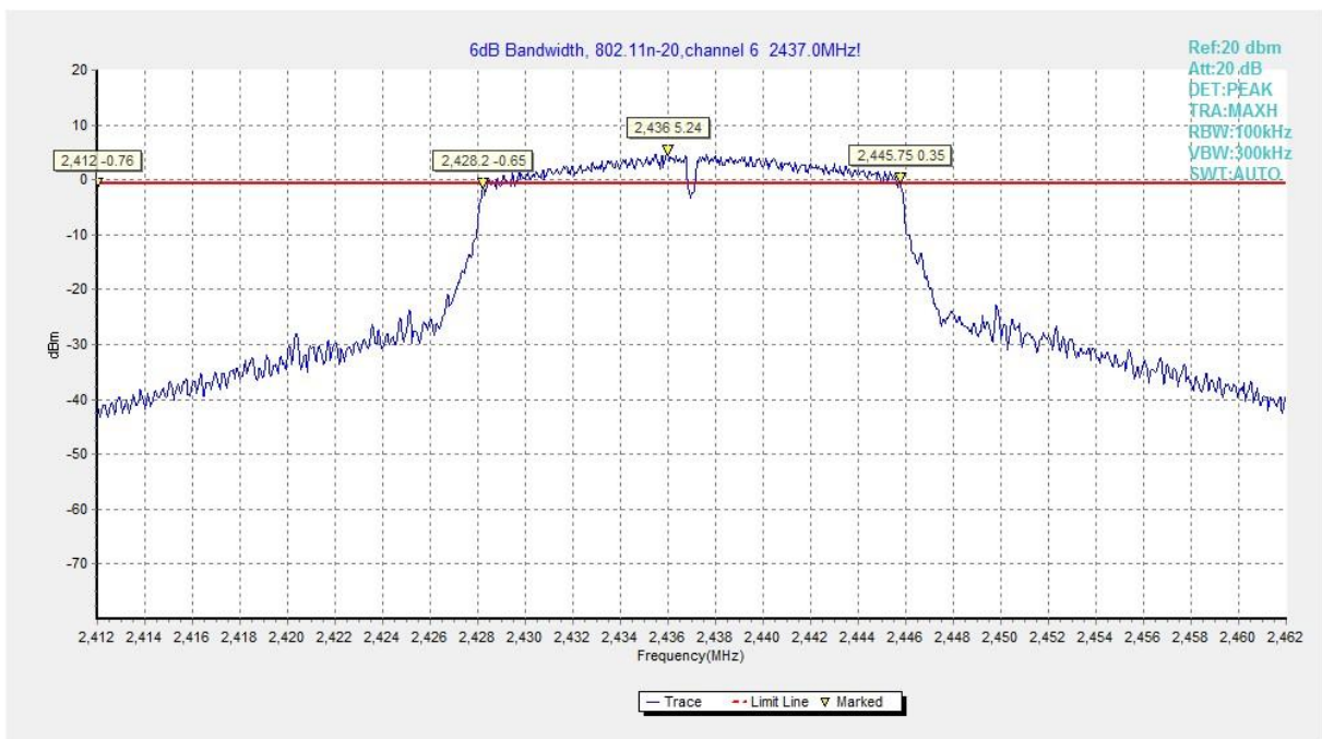
Fig.A.4.8 DTS Bandwidth (802.11n-HT20, Ch 6)
