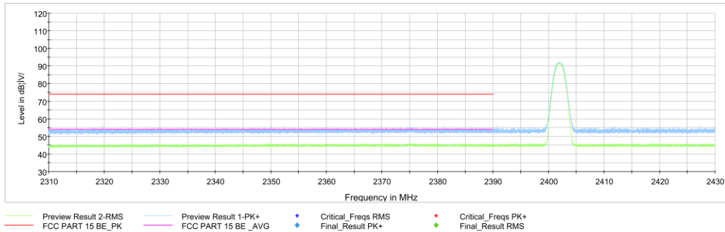
Fig.18. Frequency Band Edges: GFSK, 2402 MHz, Hopping Off, 2.31 GHz – 2.43GHz
