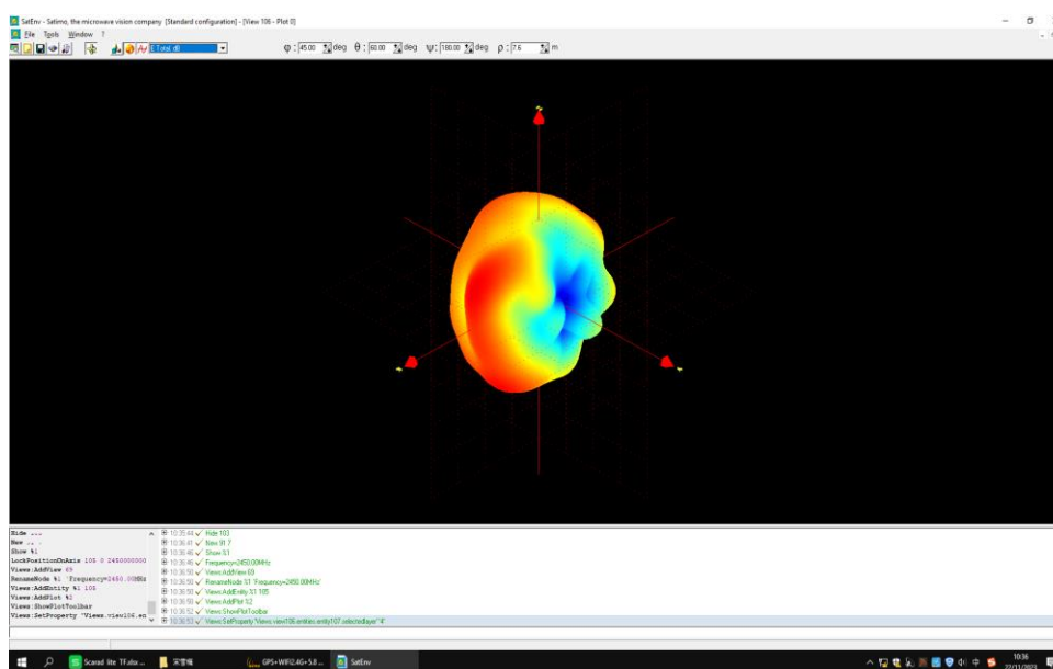
ANT 2_2450M (Frequency=2450MHz)
