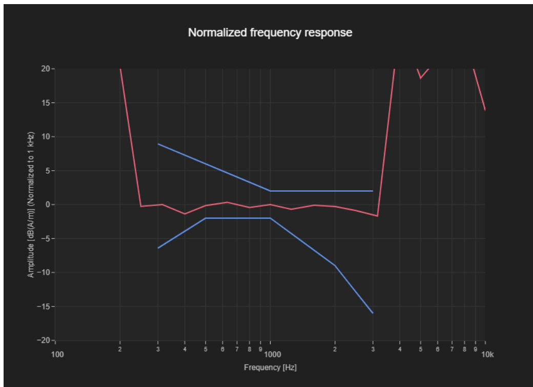
Figure.4 Frequency Response of B12-N77-OTT
