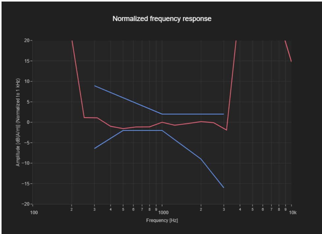
Figure.3 Frequency Response of GSM850-OTT
