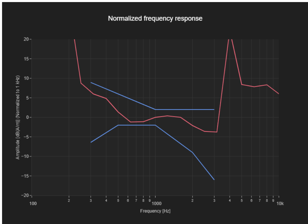
Figure.2 Frequency Response of N41
