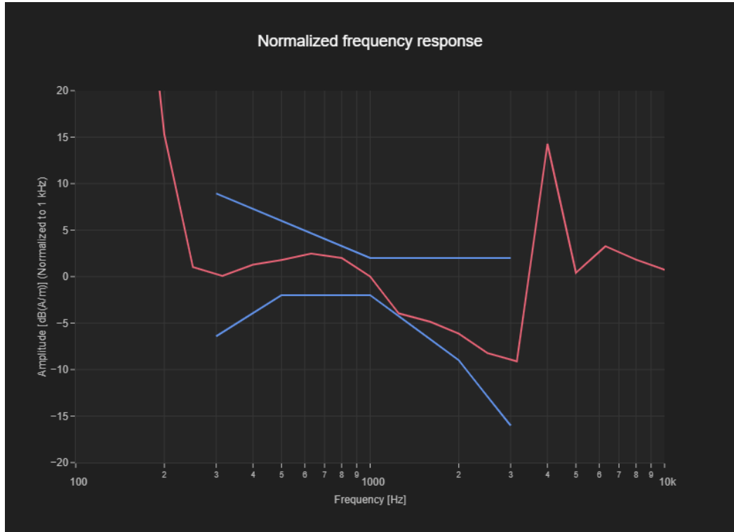
Figure.1 Frequency Response of GSM850
