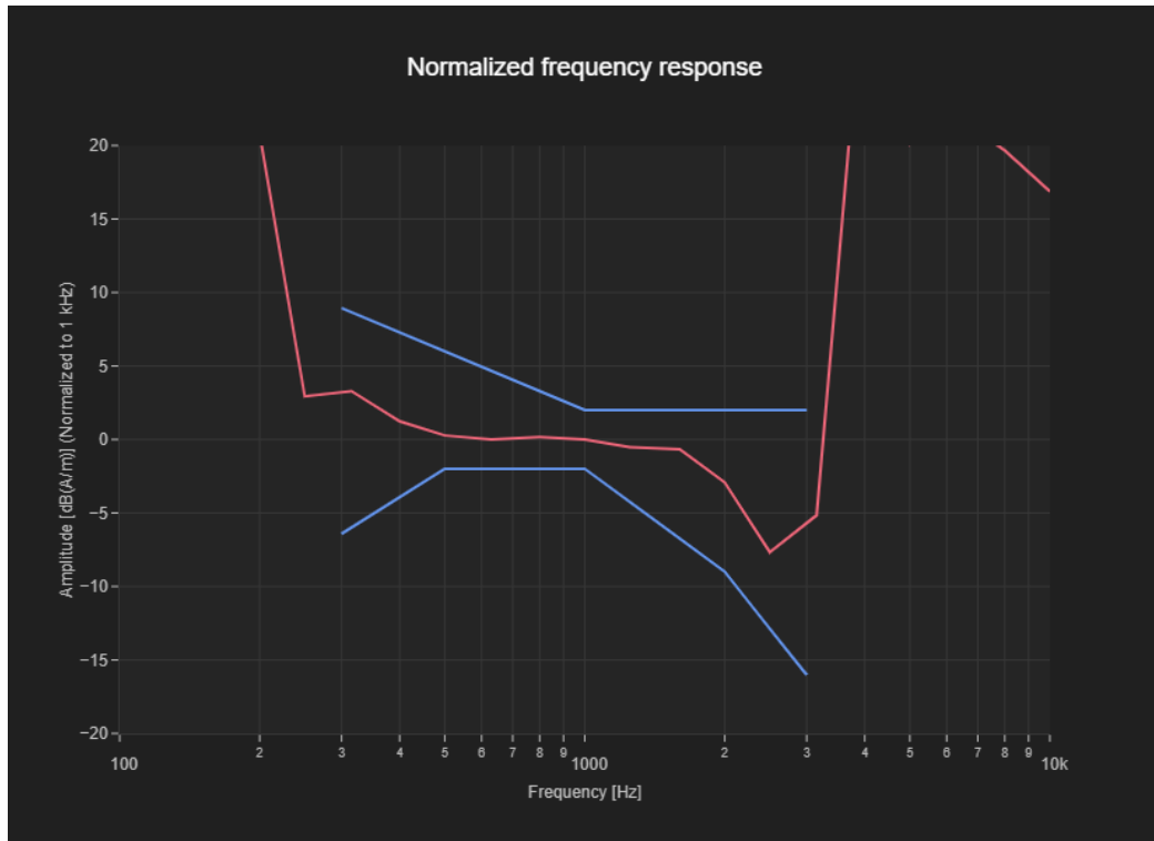
Figure C.1 Frequency Response of GSM1900
