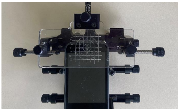
Pic 3: Handset Positioner (HHPIII) with mounted EUT mobile phone
