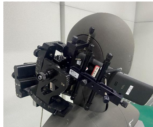
Pic 3: Handset Positioner (HHPIII) with mounted EUT mobile phone
