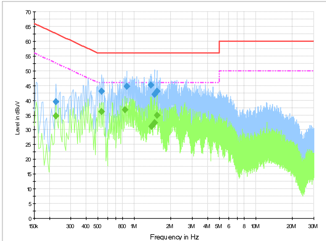
Fig.B.10.1 AC Powerline Conducted Emission- bluetooth
