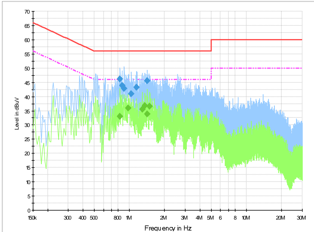
Fig.B.8.2 AC Powerline Conducted Emission-Idle
