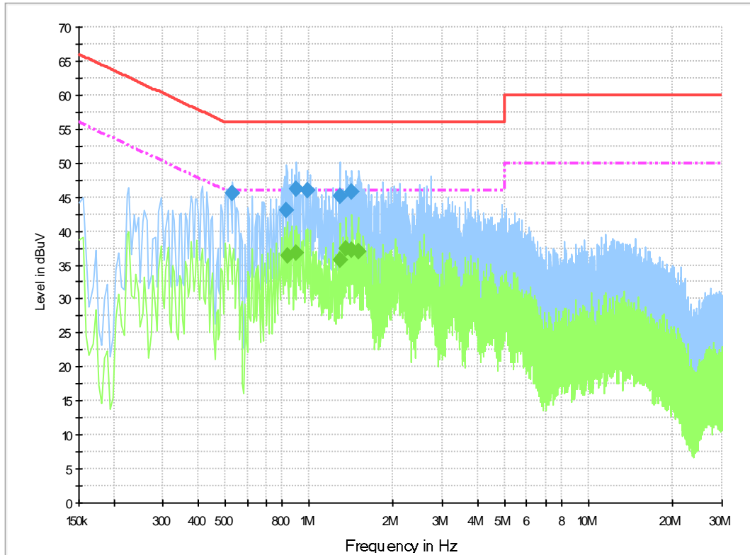
Fig.B.8.1 AC Powerline Conducted Emission- bluetooth
