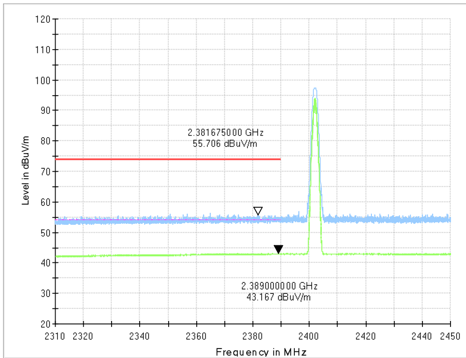
Fig.18. Frequency Band Edges: GFSK, 2402 MHz, Hopping Off, 2.31 GHz – 2.45GHz
