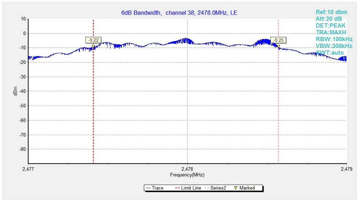
Fig.22. 6dB Bandwidth: GFSK, 2478 MHz
