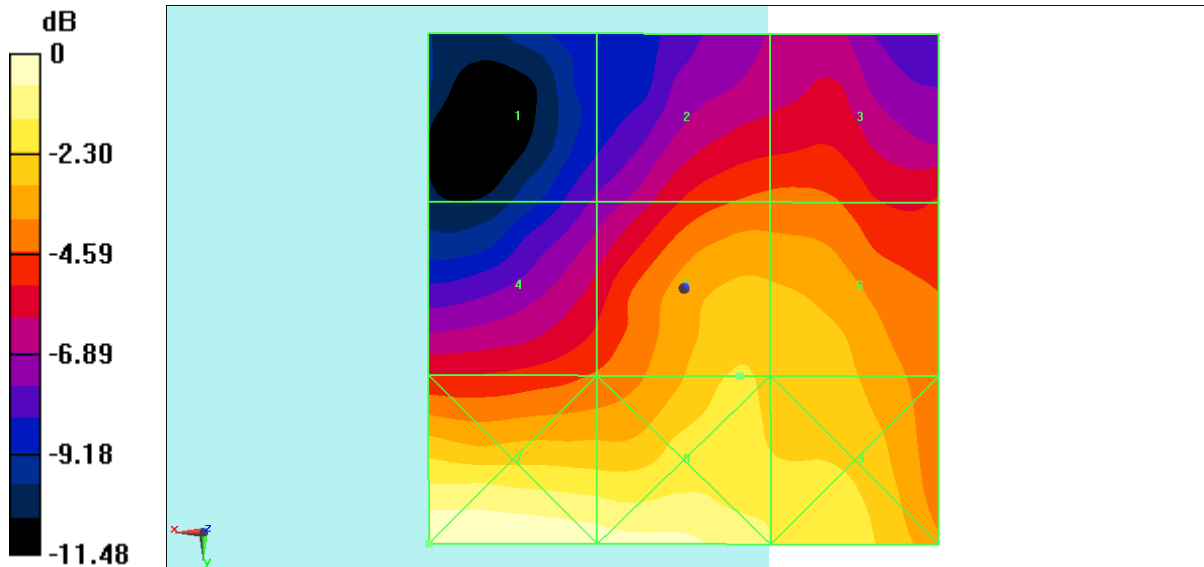
Fig B.3HAC RF E-Field WiFi2.4G
