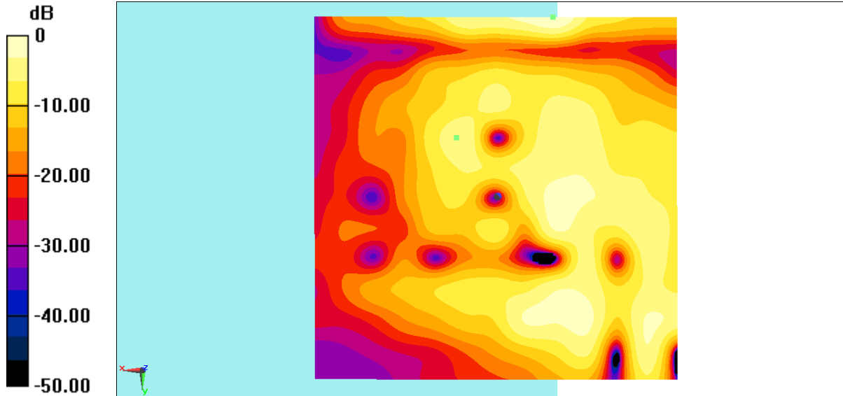
Fig B.3 T-Coil GSM1900 -OTT
