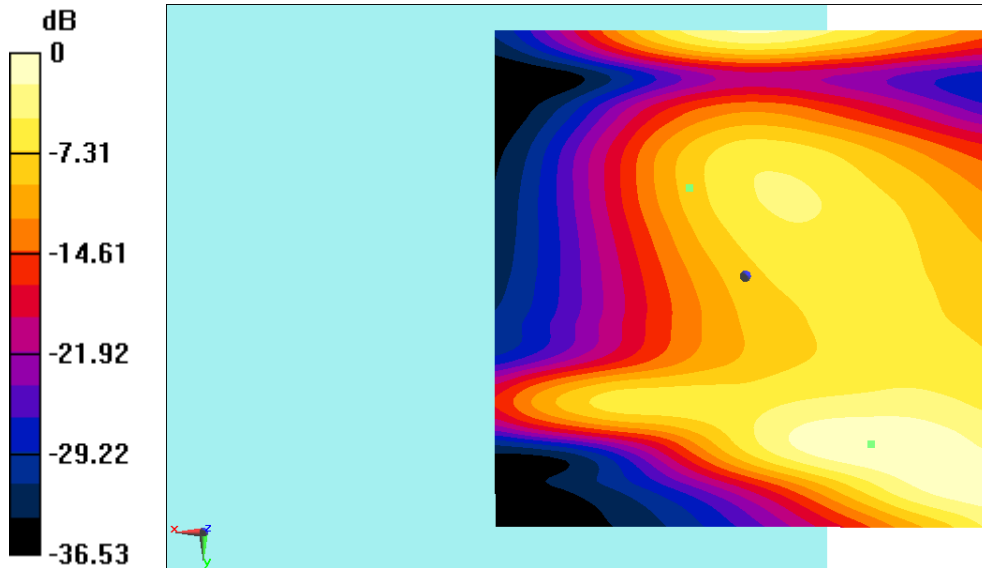
Fig B.1 T-Coil GSM850
