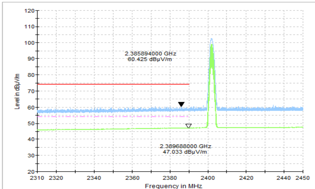
Fig.15. Frequency Band Edges: π/4 DQPSK, Channel 0, Hopping Off, 2.31 GHz - 2.45GHz
