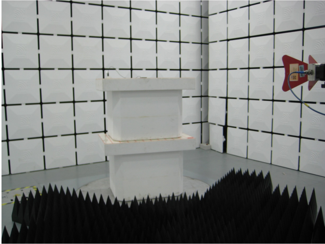
Above 1GHz
