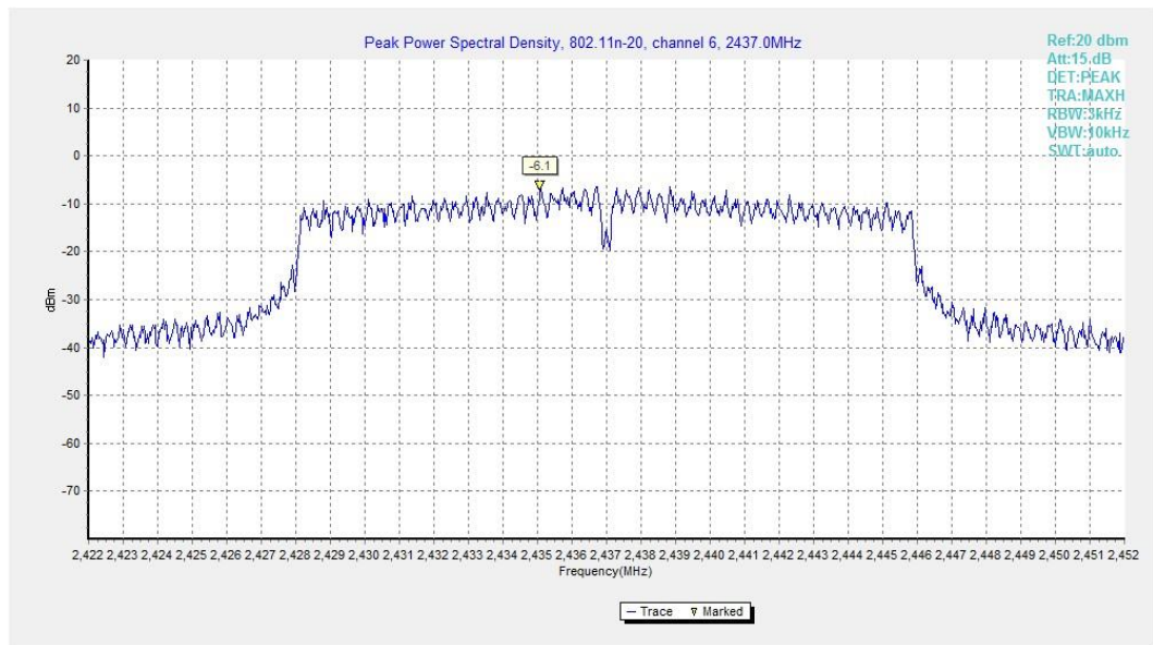
Fig.A.3.8 Power Spectral Density (802.11n-HT20, Ch 6)
