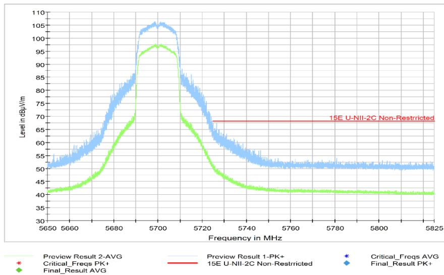
Fig.49 Band Edges (802.11ac-HT20 Ch140, 5700MHz)
