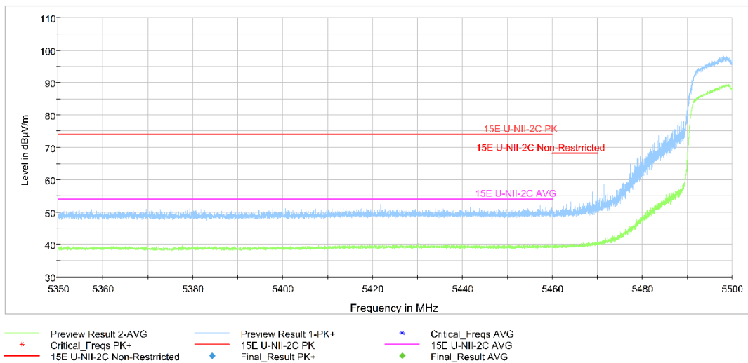
Fig.48 Band Edges (802.11ac-HT20 Ch100, 5500MHz)
