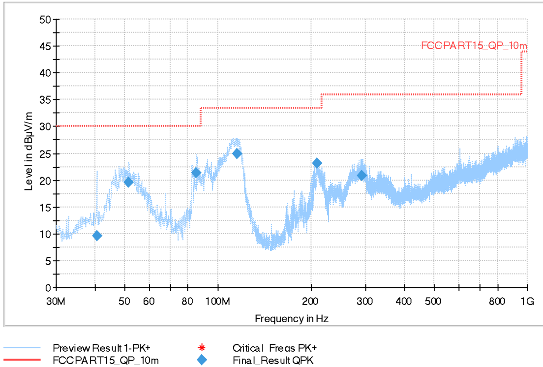
Figure B-6: Measurement results for Electric Field Radiated Emissions ( \geq 30\text{MHz} )
