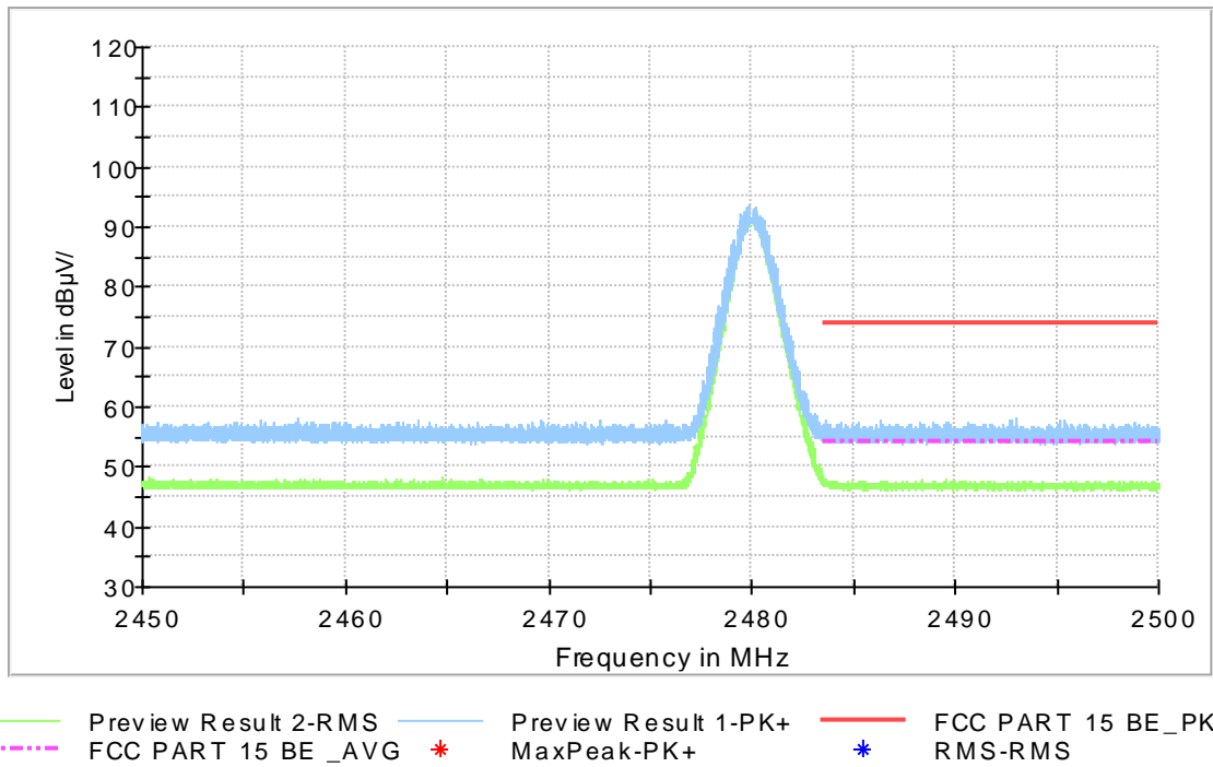
Fig.18. Frequency Band Edges: 8DPSK, Channel 78, 2.45 GHz - 2.50GHz
