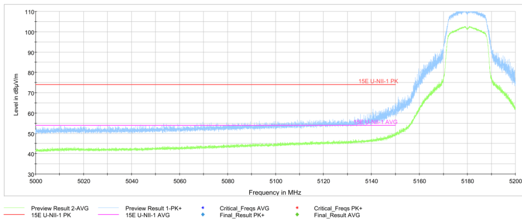
Fig.34 Band Edges (802.11a, 5180MHz)
