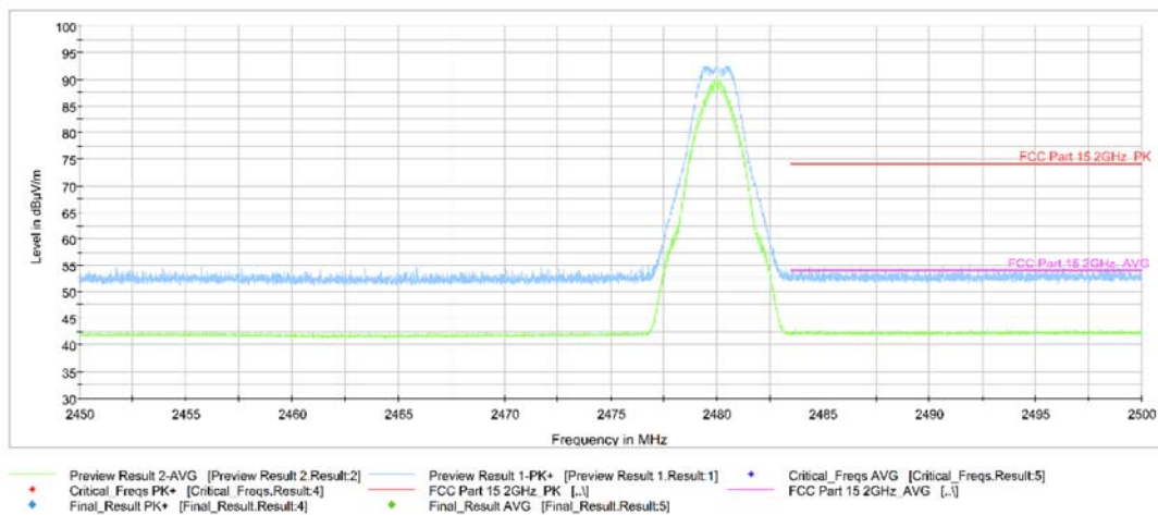
Fig.4. Frequency Band Edges: GFSK, 2480 MHz, Hopping Off , 2.45 GHz - 2.50GHz
