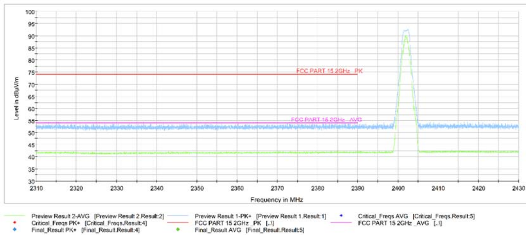
Fig.3. Frequency Band Edges: GFSK, 2402 MHz, Hopping Off, 2.31 GHz – 2.43GHz
