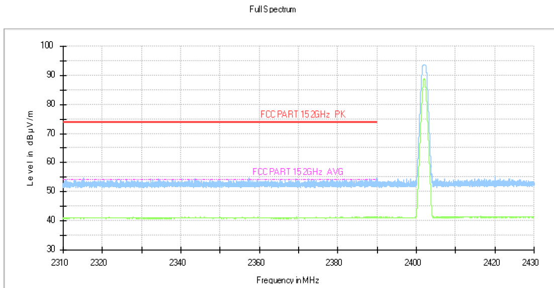
Fig.3. Frequency Band Edges: GFSK, 2402 MHz, Hopping Off, 2.31 GHz – 2.43GHz
