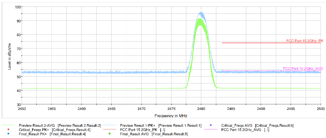
Fig.18. Frequency Band Edges: 8DPSK, Channel 78, 2.45 GHz - 2.50GHz
