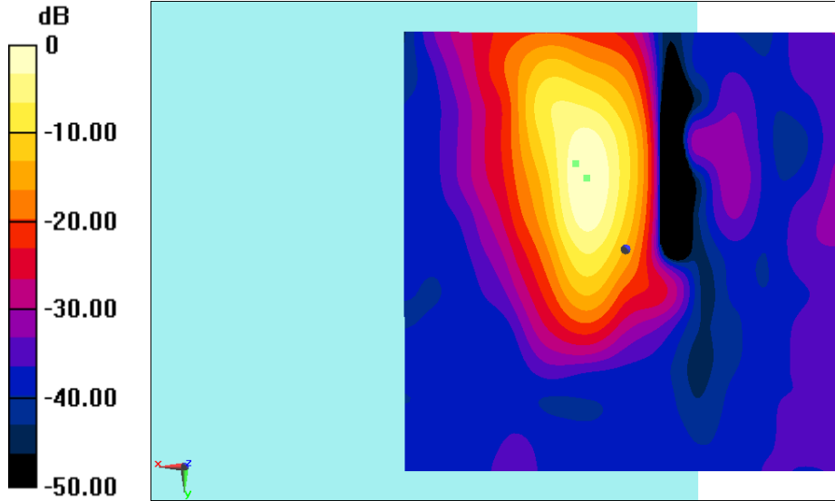
Fig B.4 T-Coil GSM850
