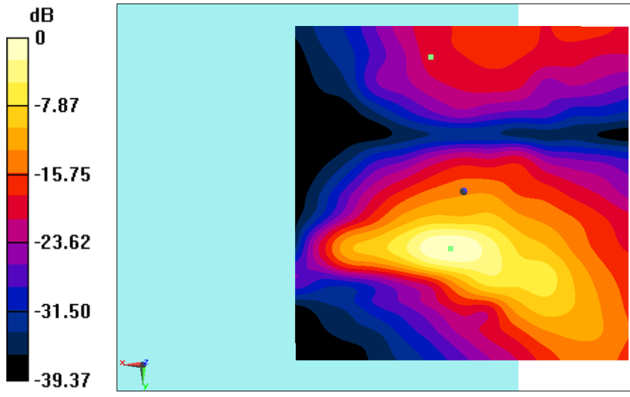
Fig B.3 T-Coil GSM850
