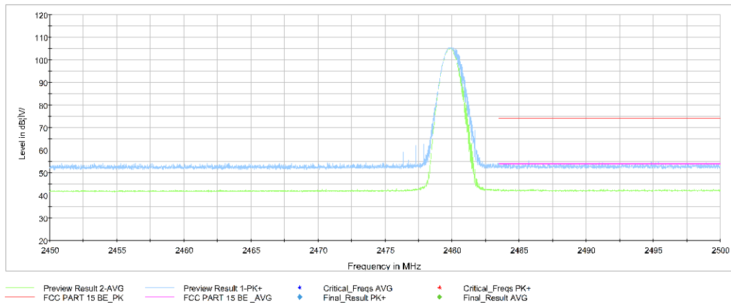
Fig.14. Frequency Band Edges: GFSK, Channel 78, Hopping Off, ch11, 2.45 GHz - 2.50GHz
