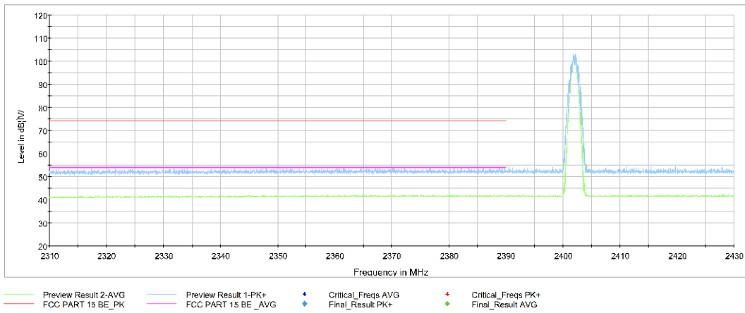
Fig.17. Frequency Band Edges: 8DPSK, Channel 0, 2.31 GHz - 2.43GHz
