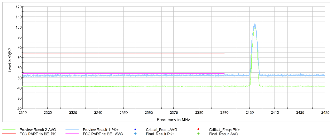
Fig.15. Frequency Band Edges: \pi/4 DQPSK, Channel 0, Hopping Off, 2.31 GHz - 2.43GHz
