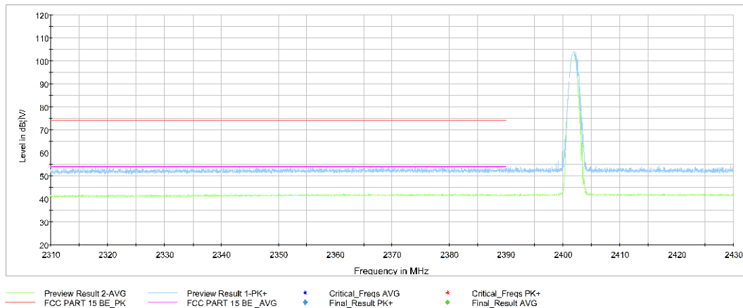
Fig.13. Frequency Band Edges: GFSK, Channel 0, Hopping Off, 2.31 GHz – 2.43GHz
