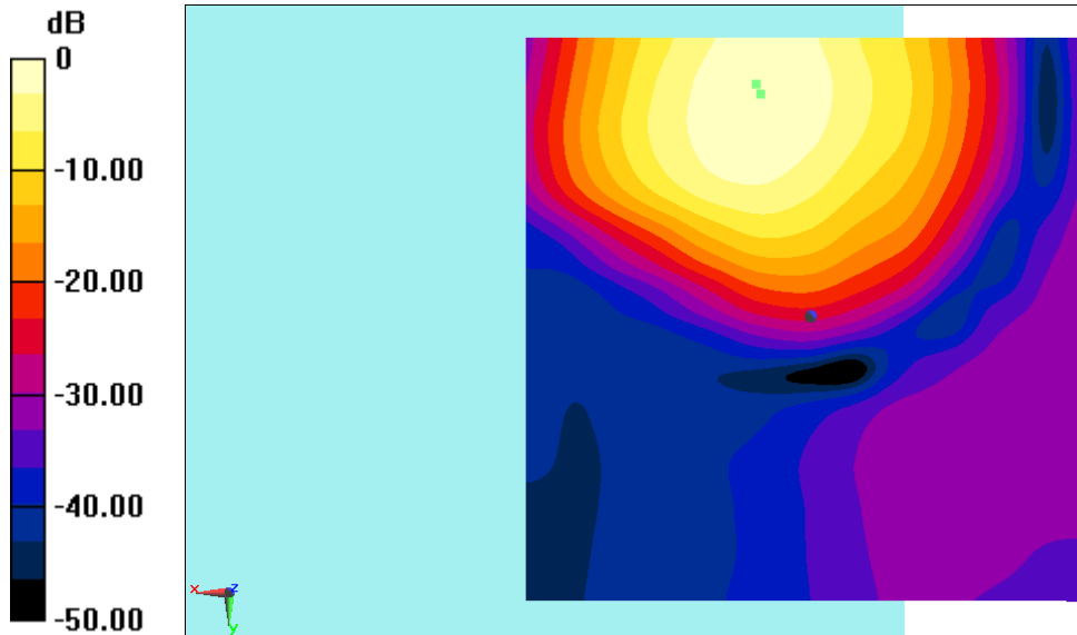
Fig B.2 T-Coil LTEB2
