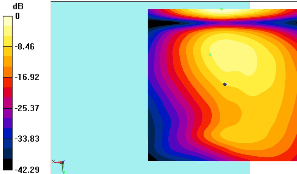
Fig B.1 T-Coil LTEB2
