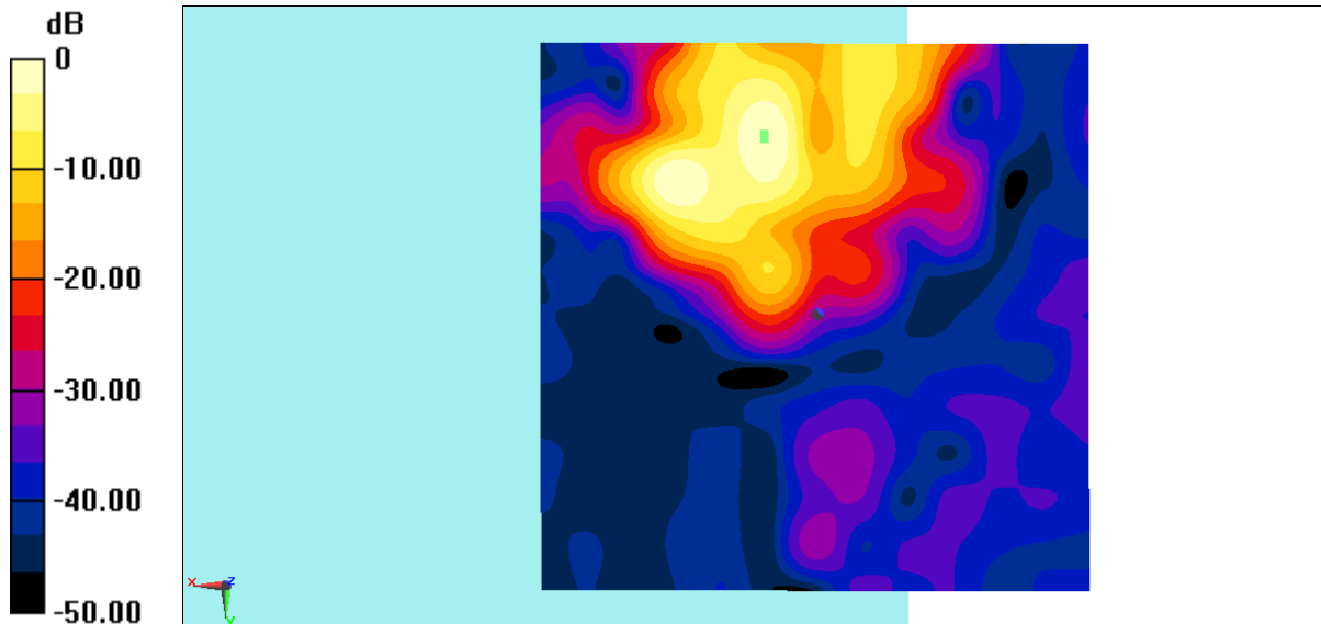
Fig B.4 T-Coil GSM1900
