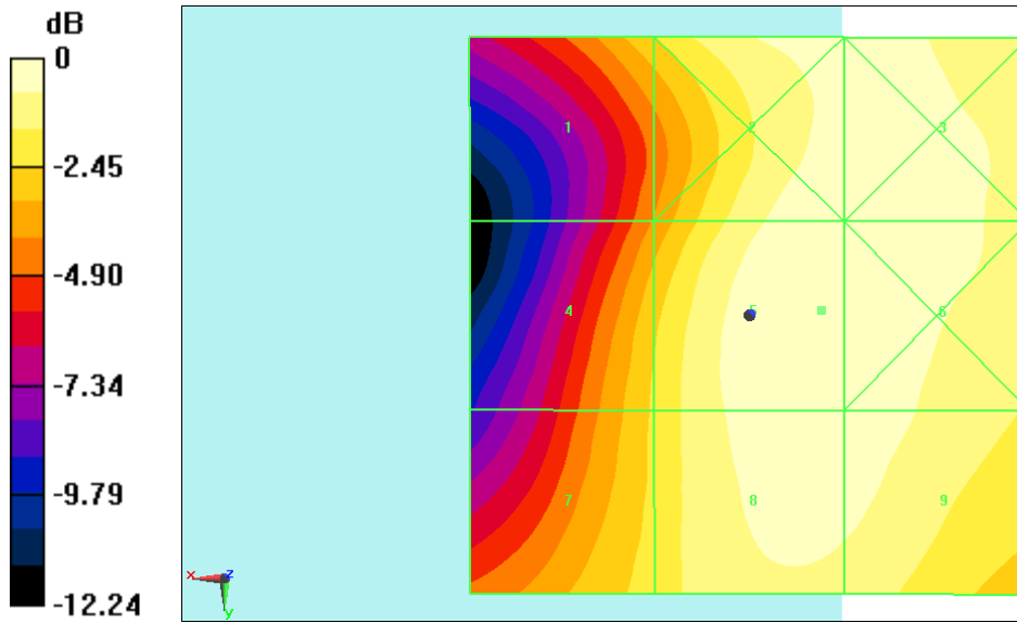
Fig B.3 HAC RF E-Field WIFI2.4G
