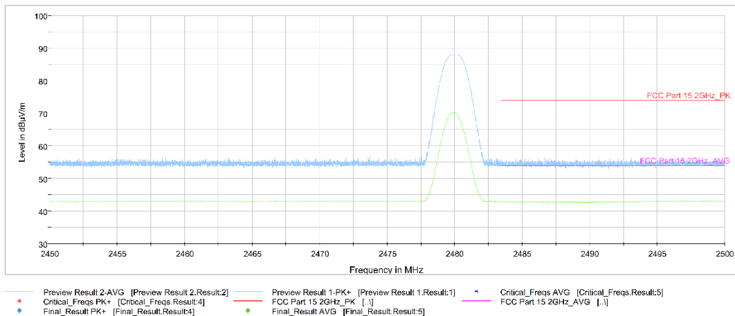
Fig.4. Frequency Band Edges: GFSK, 2480 MHz, 2.45 GHz - 2.50GHz
