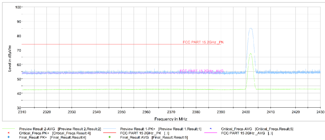
Fig.3. Frequency Band Edges: GFSK, 2402 MHz, 2.31 GHz – 2.43GHz
