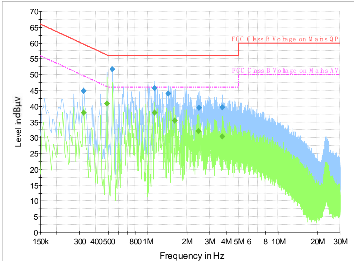
Fig.B.9.1 AC Powerline Conducted Emission- Bluetooth
