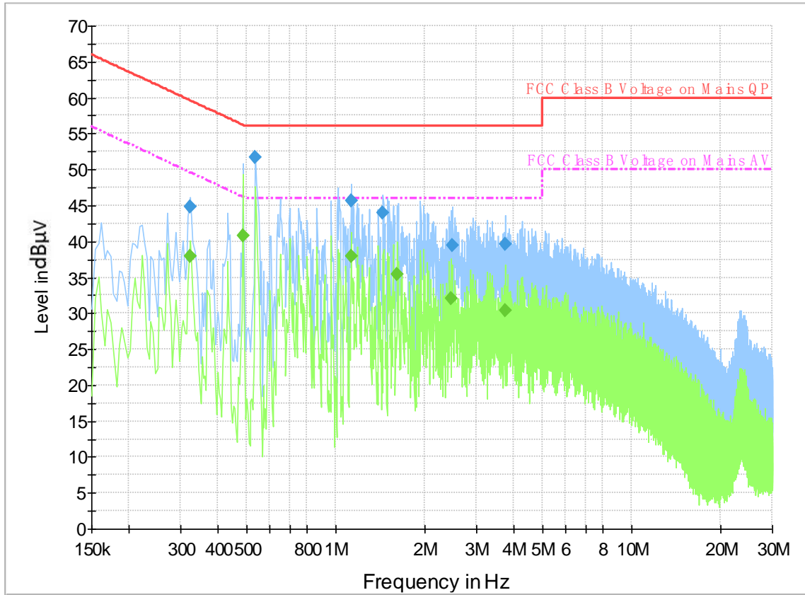
Fig.B.11.1 AC Powerline Conducted Emission- Bluetooth
