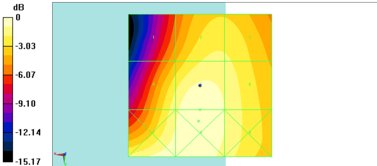
Fig B.1 HAC RF E-Field LTE Band41 PC2 16QAM CH40620
