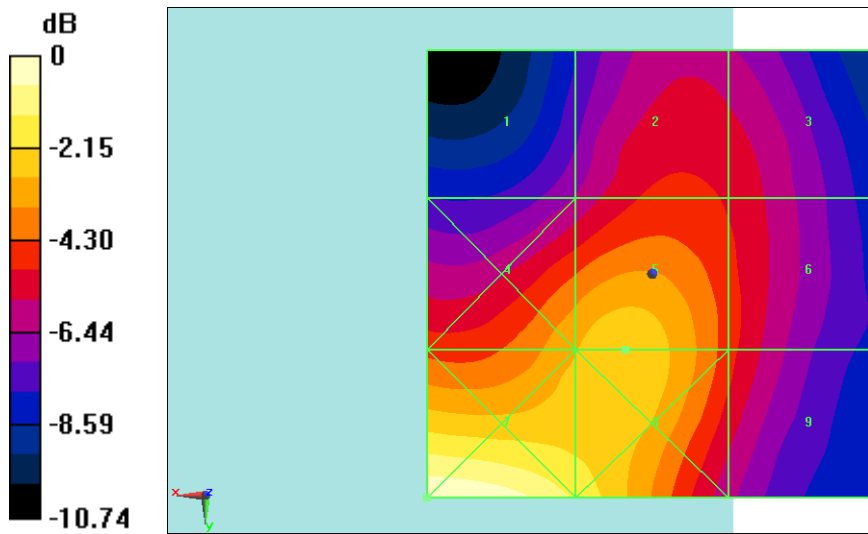
Fig B.2 HAC RF E-Field LTE Band41 PC3 QPSK CH40185
