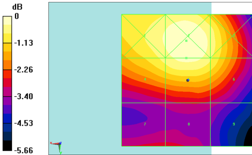
Fig B.3 HAC RF E-Field WiFi2.4G 11b
