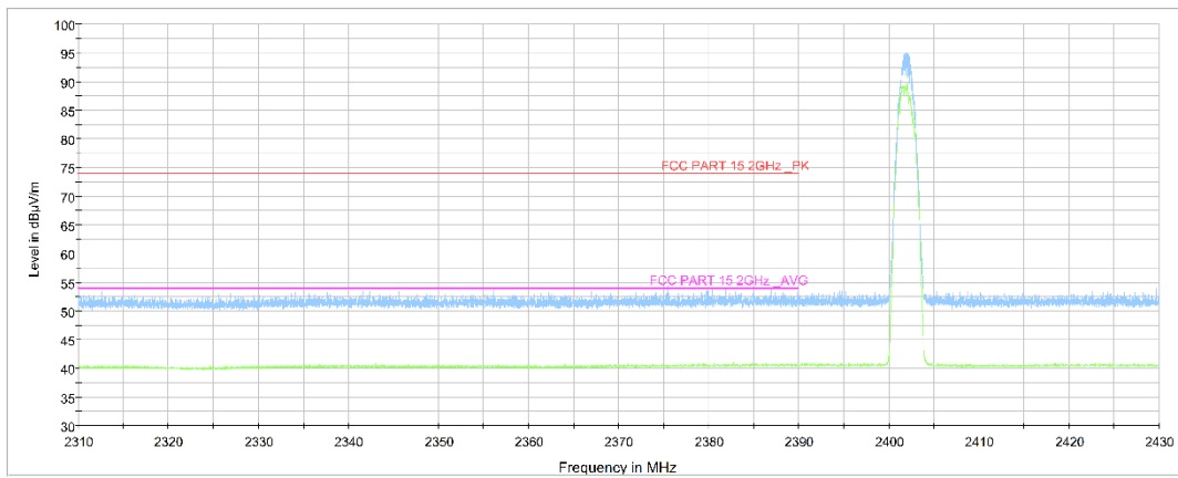
Fig.17. Frequency Band Edges: 8DPSK, Channel 0, 2.31GHz ~2.43GHz
