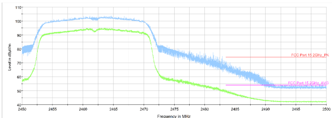
Fig.A.6.2.6 Transmitter Spurious Emission - Radiated (Power): 802.11n-HT20, ch11, 2.45 GHz - 2.50GHz
