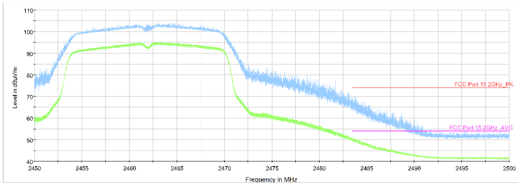
Fig.A.6.2.4 Transmitter Spurious Emission - Radiated (Power): 802.11g, ch11, 2.45 GHz - 2.50GHz
