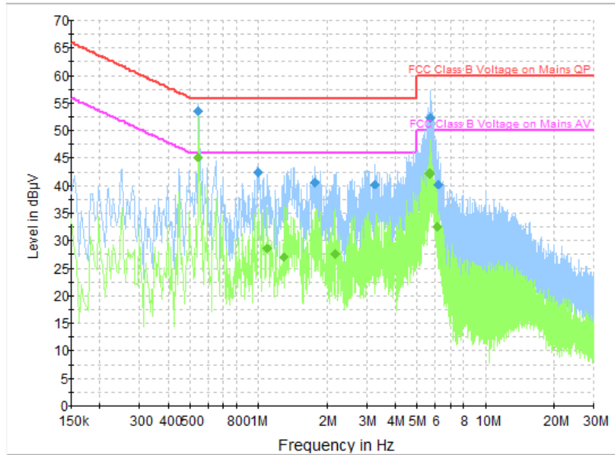
Fig.B.9.2 AC Powerline Conducted Emission-Idle
