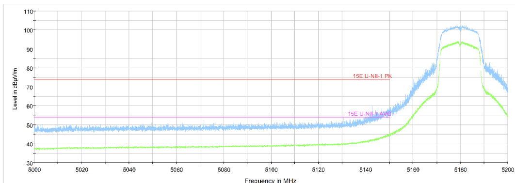
Fig.34 Band Edges (802.11a Ch36, 5180MHz)
