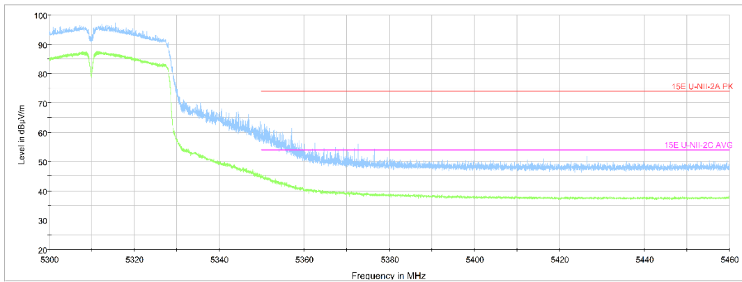
Fig.51 Band Edges (802.11ac-HT40 Ch62, 5310MHz)
