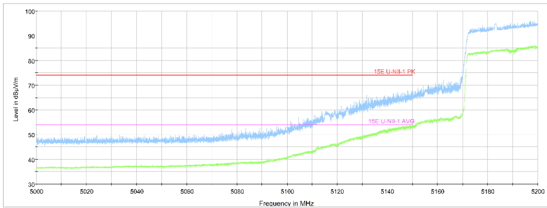
Fig.54 Band Edges (802.11ac-HT80 Ch42 , 5210MHz)
