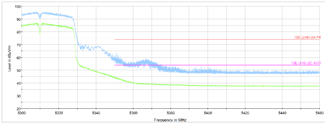
Fig.43 Band Edges (802.11n-HT40 Ch62, 5310MHz)
