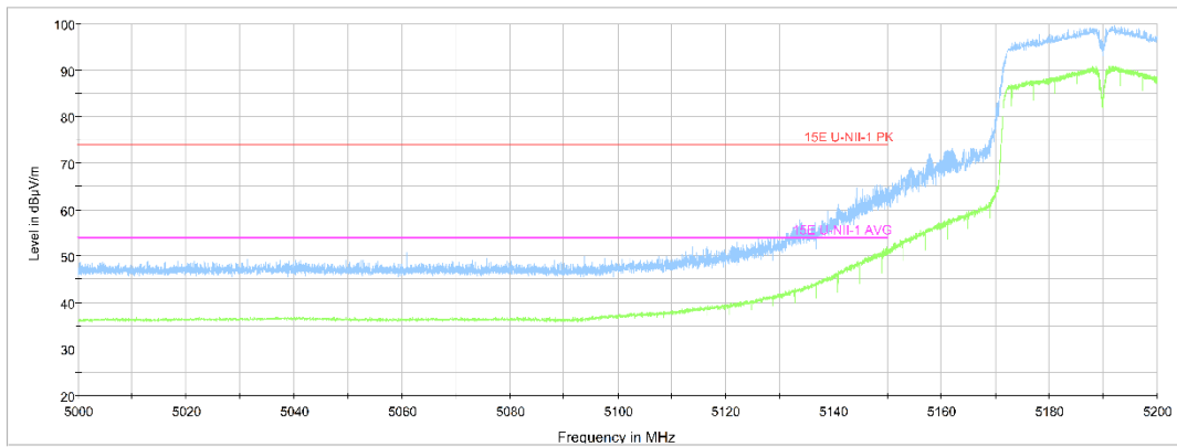
Fig.42 Band Edges (802.11n-HT40 Ch38, 5190MHz)
