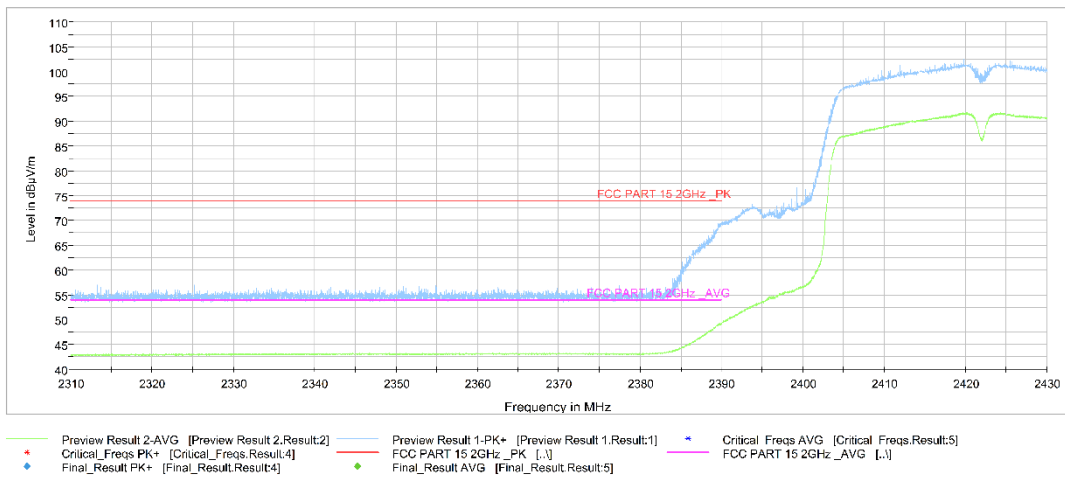
Fig.A.6.2.7 Transmitter Spurious Emission - Radiated (Power): 802.11n-HT40, ch3, 2.31 GHz - 2.43GHz
