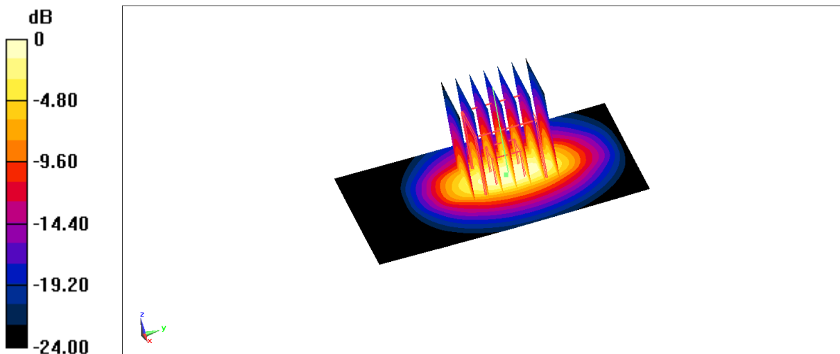
Fig.B.19 validation 2600 MHz 250mW
