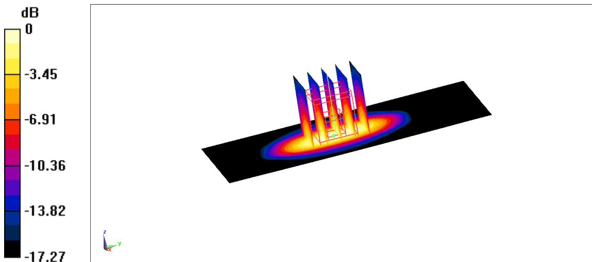
Fig.B.9 validation 1750 MHz 250mW
