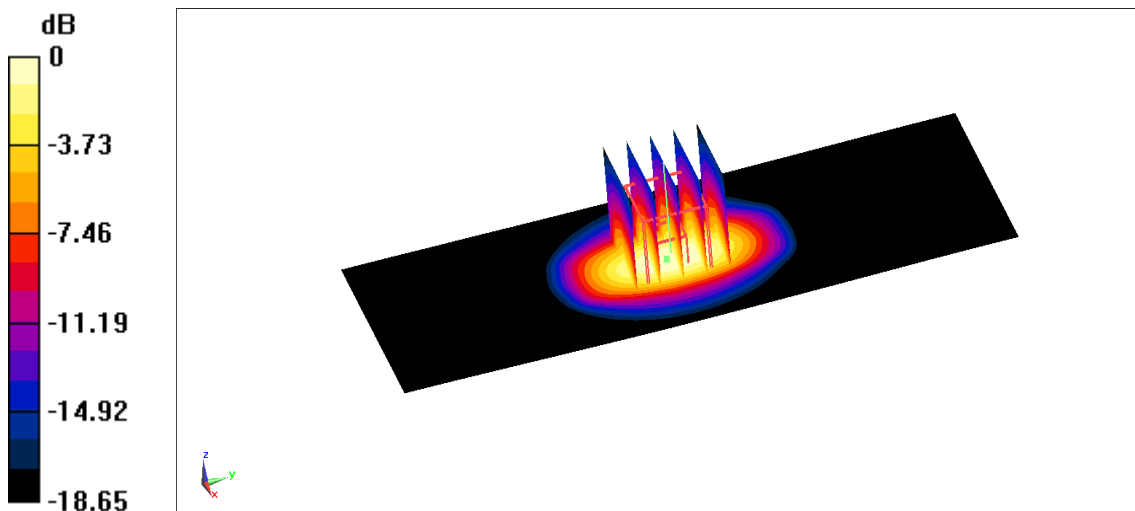
Fig.B.13 validation 1900 MHz 250mW
