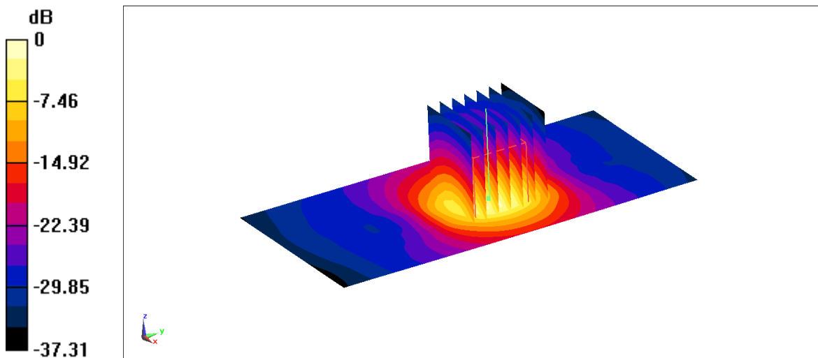
Fig.B.17 validation 2450 MHz 250mW
