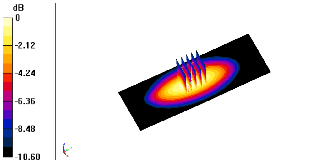
Fig.B.5 validation 835 MHz 250mW
