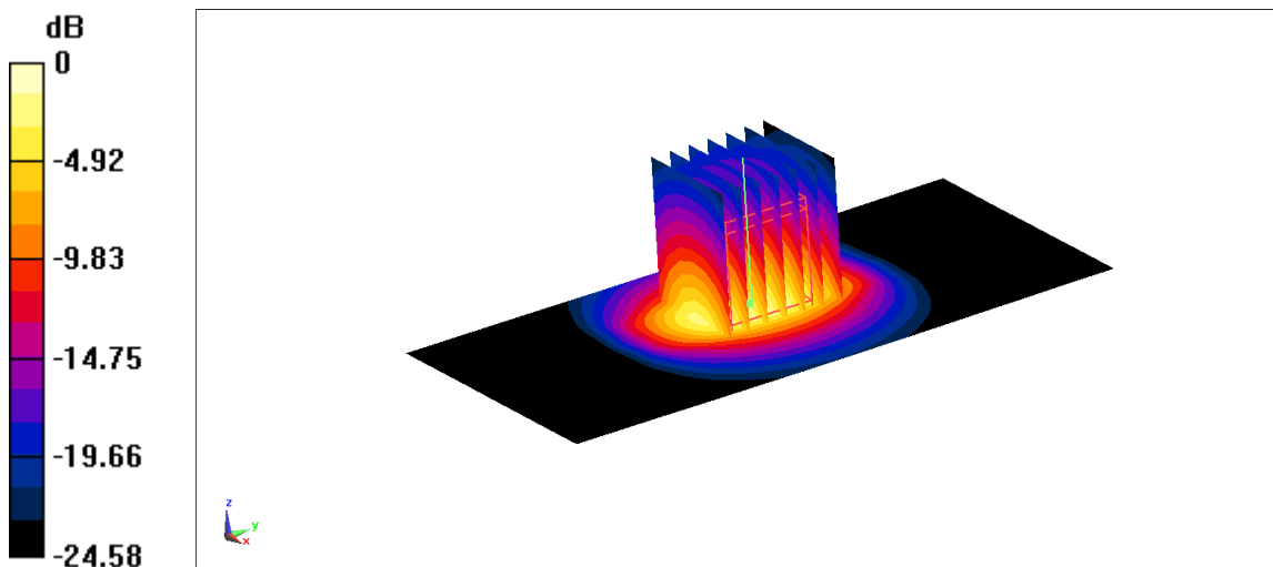
Fig.B.19 validation 2600 MHz 250mW
