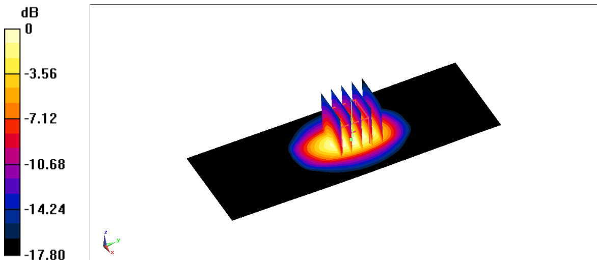
Fig.B.7 validation 835 MHz 250mW
