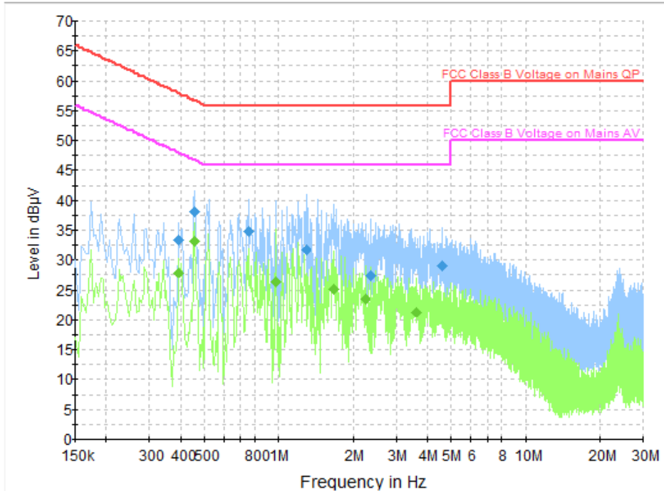
Fig.B.11.1 AC Powerline Conducted Emission- bluetooth
