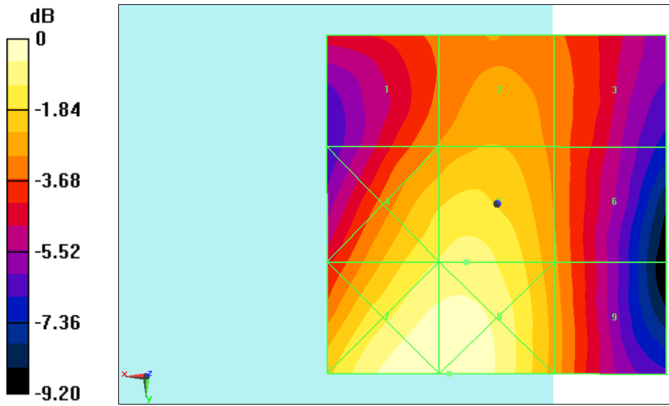
Fig B.2 HAC RF E-Field GSM 1900 Middle
