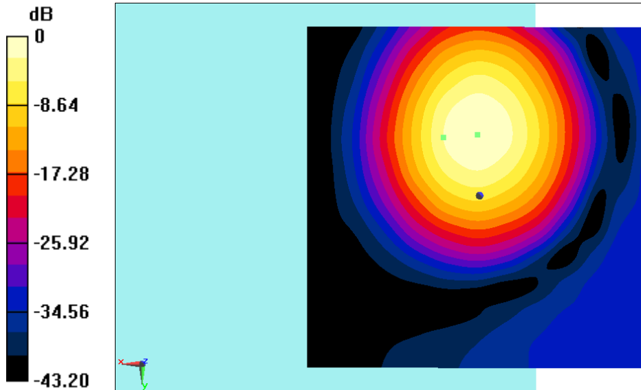
Fig B.2 T-Coil GSM850
