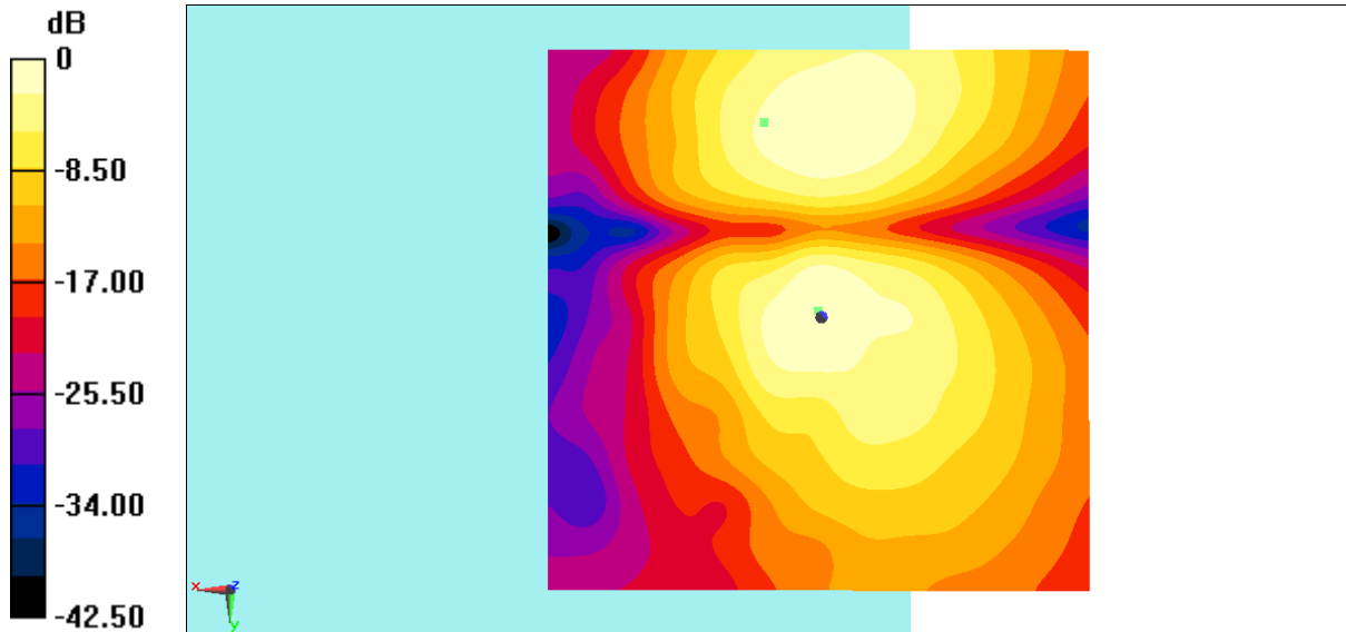
Fig B.1 T-Coil LTEBand 7
