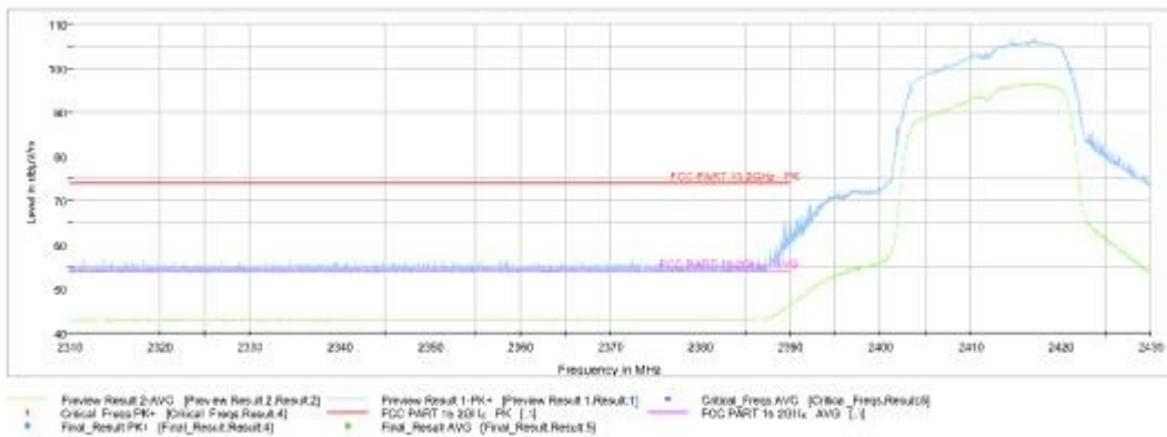
Fig.A.6.2.5 Transmitter Spurious Emission - Radiated (Power): 802.11n-HT20, ch1, 2.31 GHz - 2.43GHz
