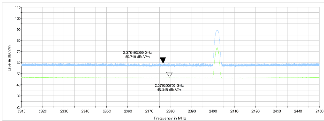
Fig.3. Frequency Band Edges: GFSK, 2402 MHz, Hopping Off, 2.31 GHz – 2.45GHz
