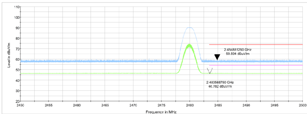
Fig.4. Frequency Band Edges: GFSK, 2480 MHz, Hopping Off, 2.45 GHz - 2.50GHz
