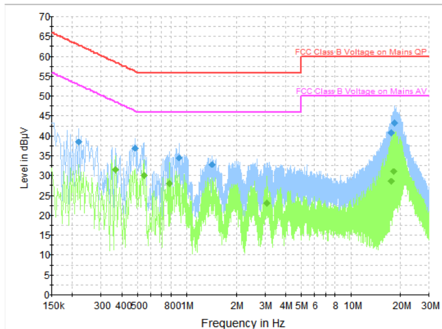
Fig.B.9.2 AC Powerline Conducted Emission-Iidle
